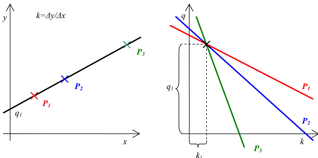
Obr. 8.8: Houghov priestor
