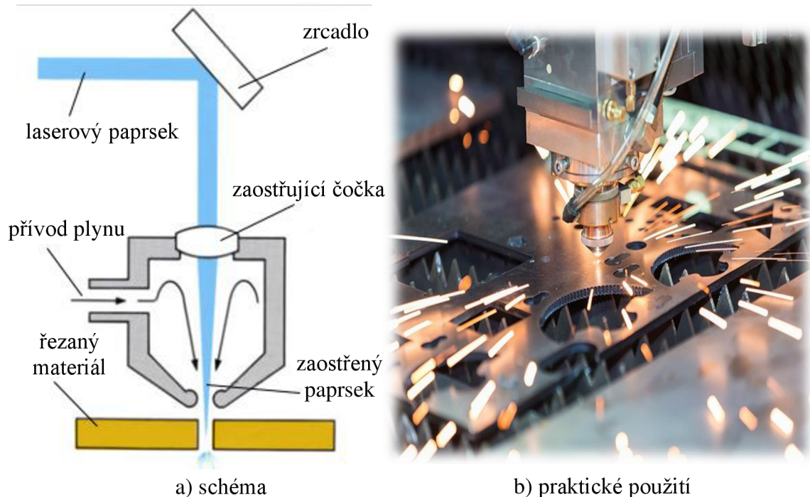
Obr. 5 Laser [9; 10].
