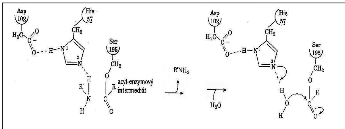
Obr. 3 Tvorba intermediátu acyl-enzym [7]
