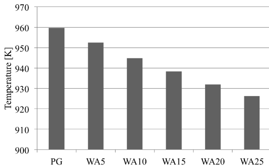
Figure 10 The effect of water injection on the in-cylinder temperature of the suction gas at the end of fuel injection (680°C - Crank Angle) [21]
