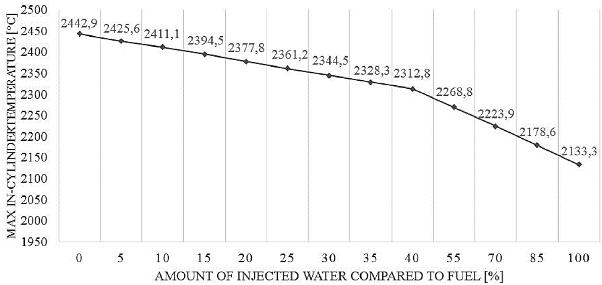
Figure 16 Decrease of maximum in-cylinder temperature
