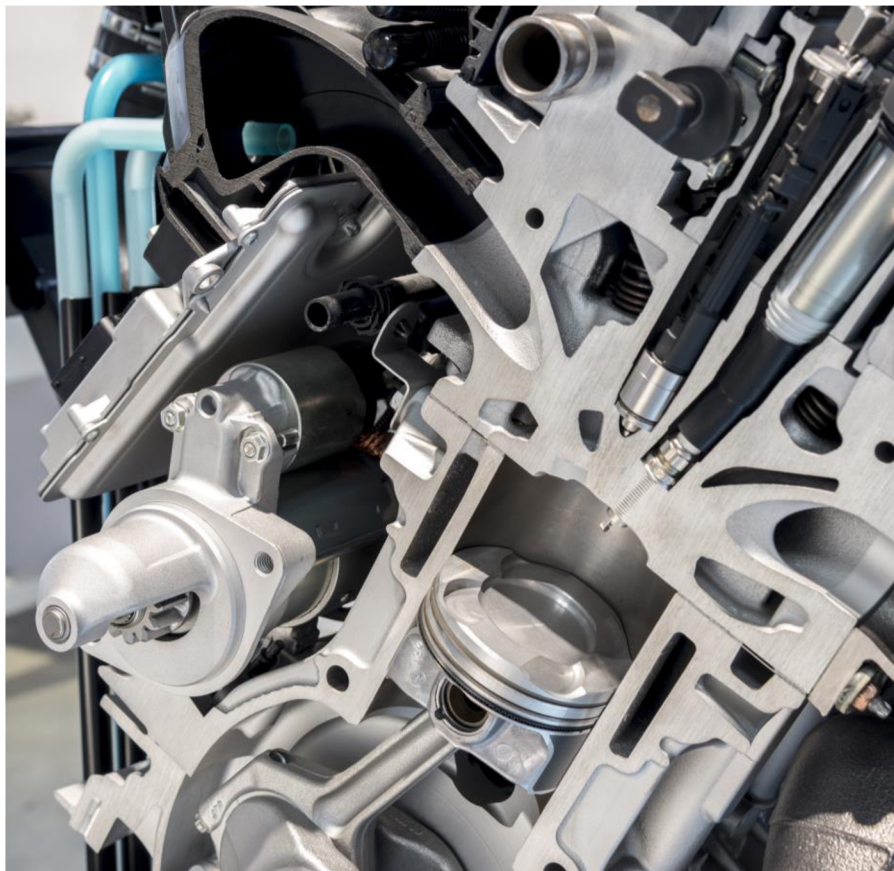
Figure 11 BMW 1-series 1,5 litre prototype engine with water injection [32]
