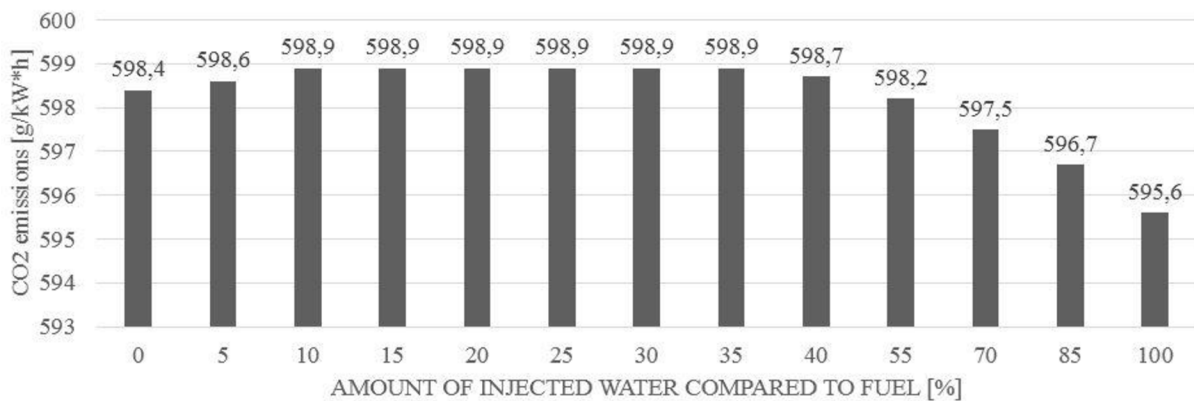
Figure 26 Change of CO 2 emissions
