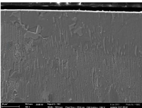
Fig. 43. Recrystallization (a) and layer of nitrides on the surface (b)
