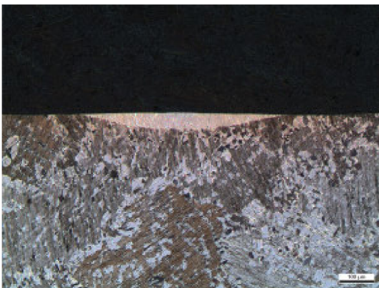
Fig. 42. Sample 12.2. Diameter = 2 mm, speed = 2000 mm/min, gas flow = 40 l/min, power = 1 kW
