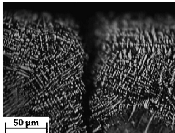
Fig. 46. Top view showing crack in some of the processed layer [19]
