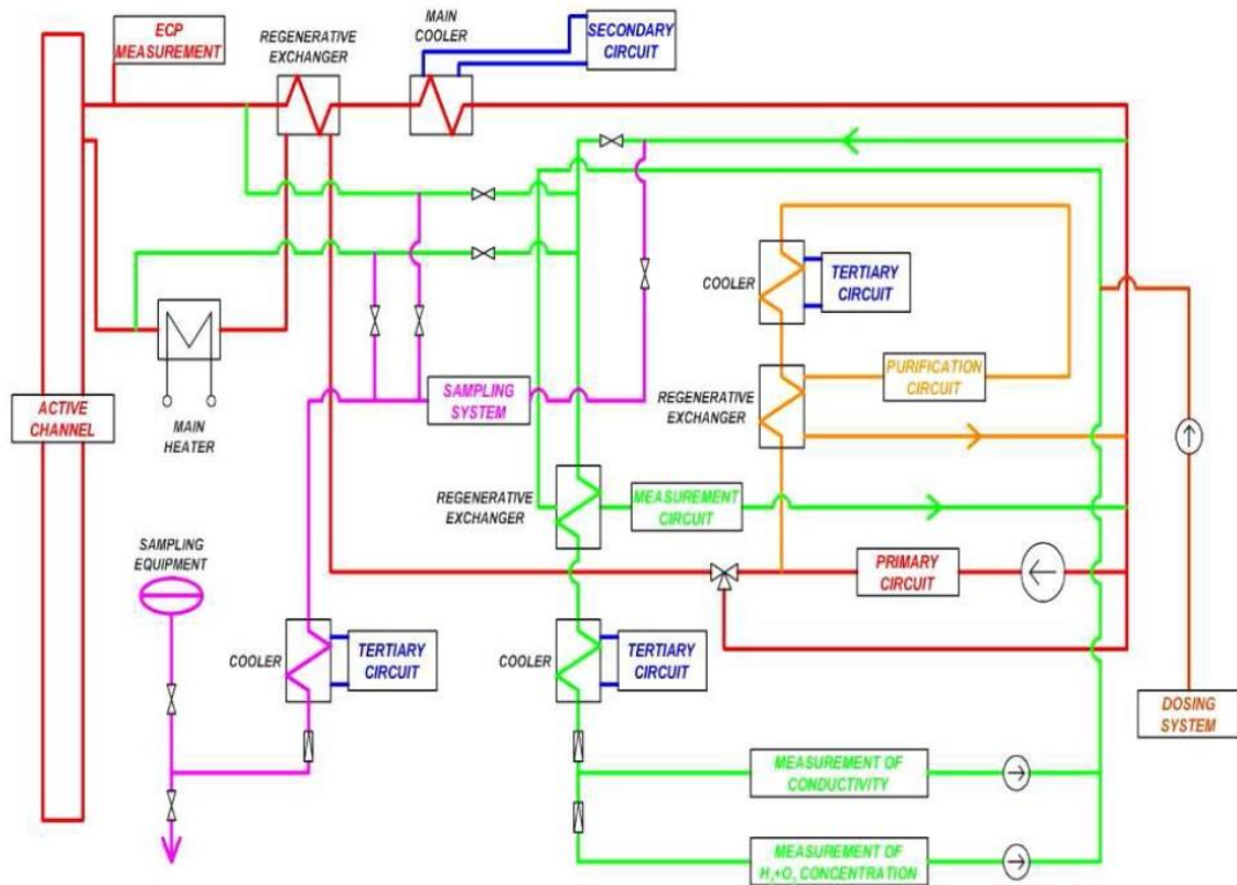
Figure 17: SCWL scheme [17]
