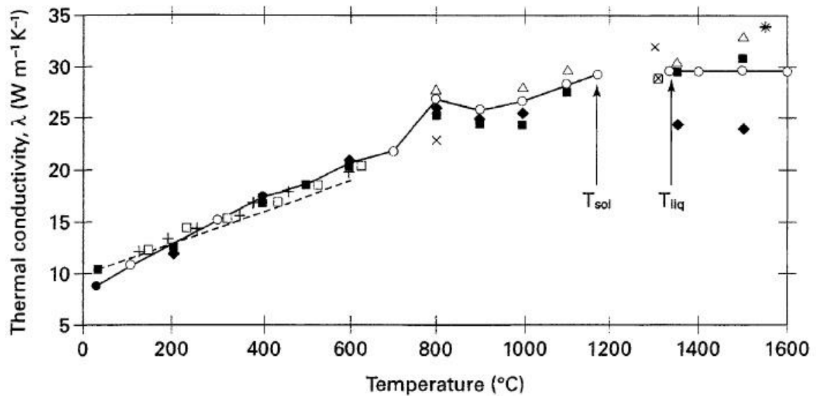
Figure 31: Thermal conductivity of Inconel 718 as a function of temperature [15]
