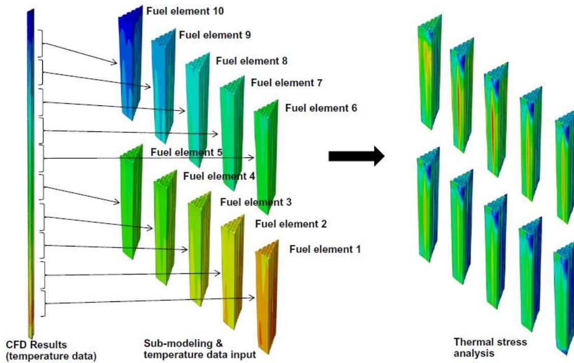
Figure 12: Sub-modeling procedure [13]
