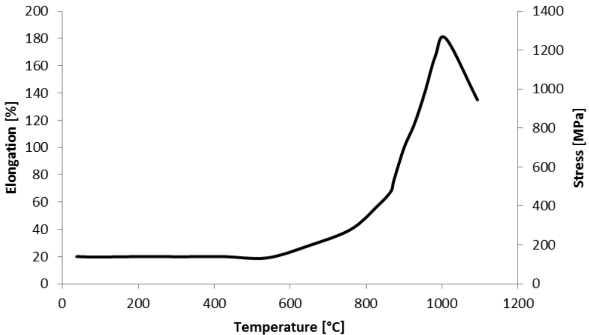
Figure 27: Stress-elongation curve depended on temperature [25]
