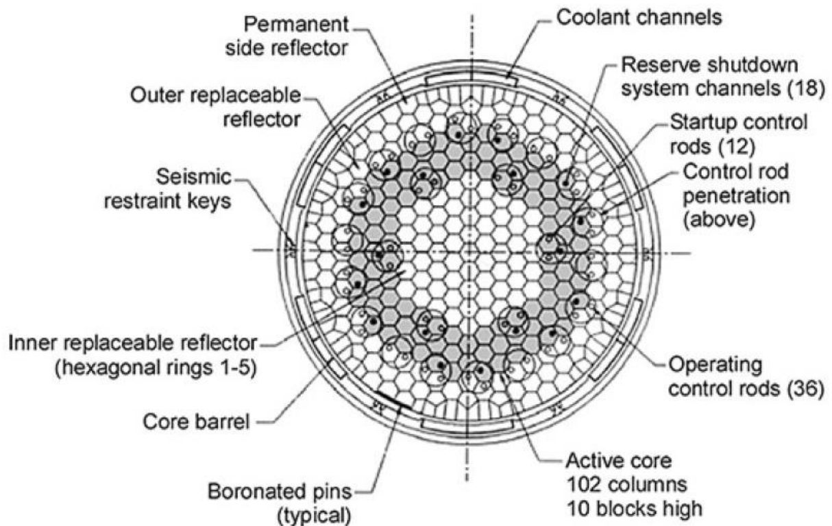
Figure 2: Prismatic core design [5]
