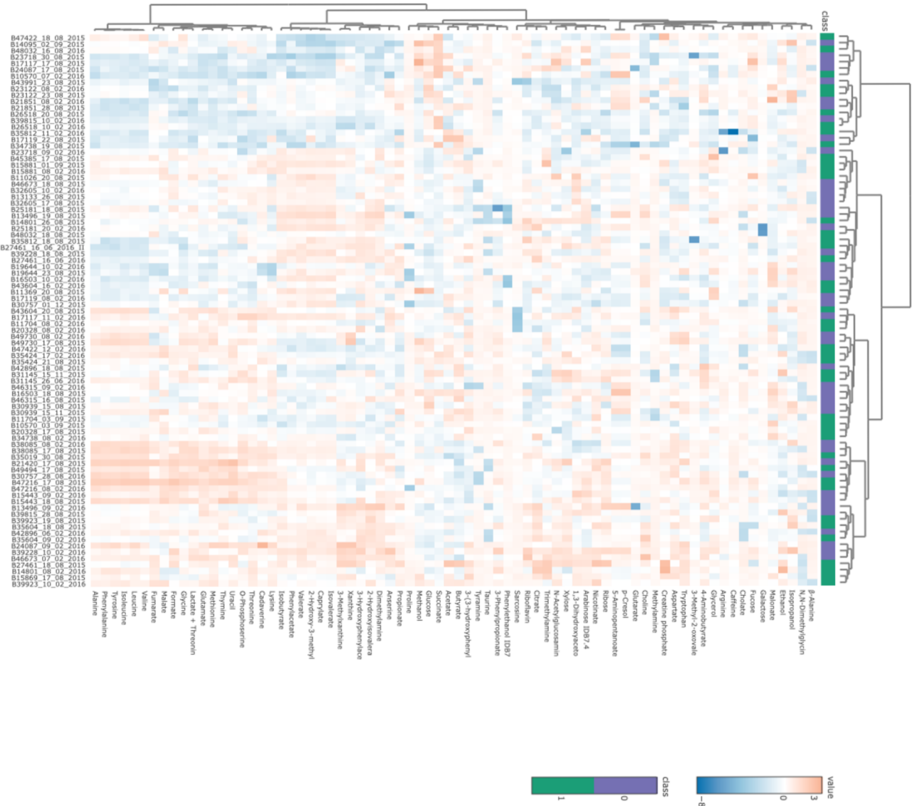
Figure 10 Heatmap based on metabolite % relative abundance.
