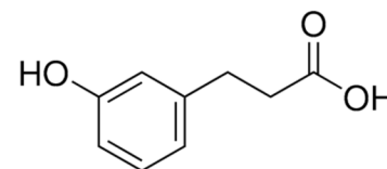
Figure 9. 3-(3-hydroxyphenyl)propionic acid skeletal formula
