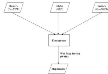
Fig 17: Schematic representation of overall workflow of preparing data for next step
