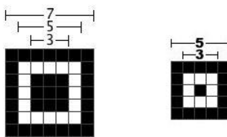
Obrázok 3.5 Finder pattern a Alignment pattern [15]
