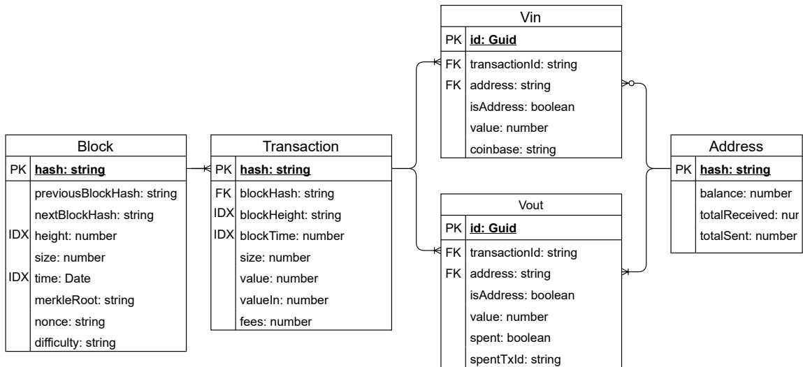
Figure 4.4: Entity-relationships diagram
