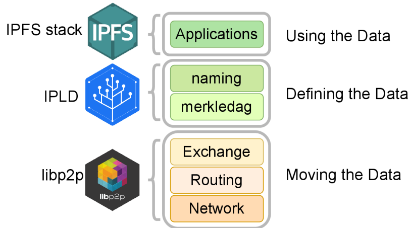
Figure 3.3: IPFS stack
