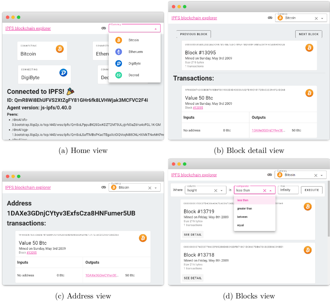
Figure 5.9: ExplorerGUI views
