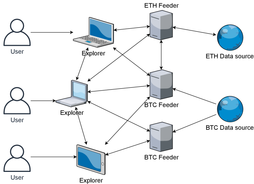
Figure 4.3: Platform architecture
