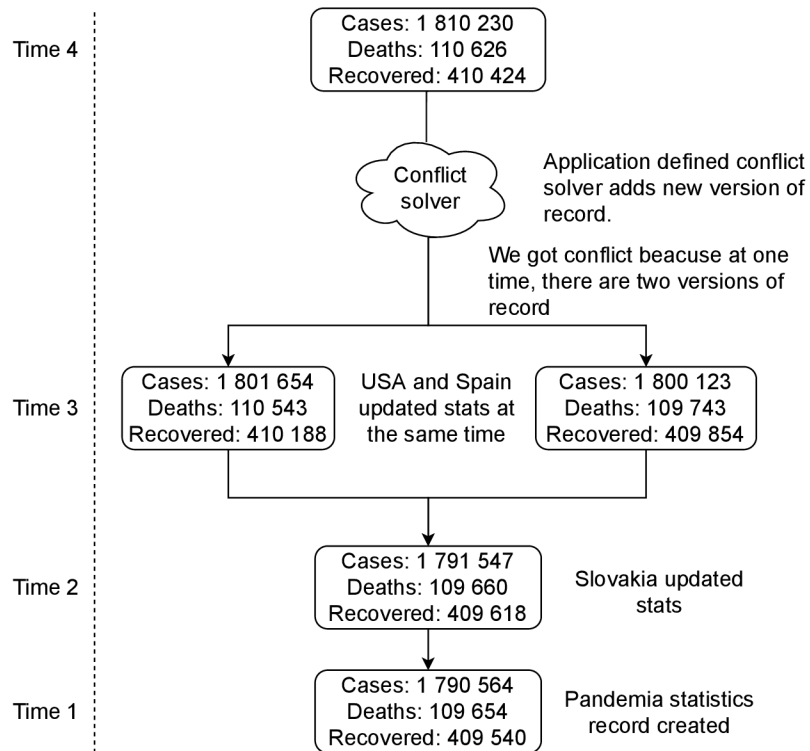
Figure 4.1: Record conflict
