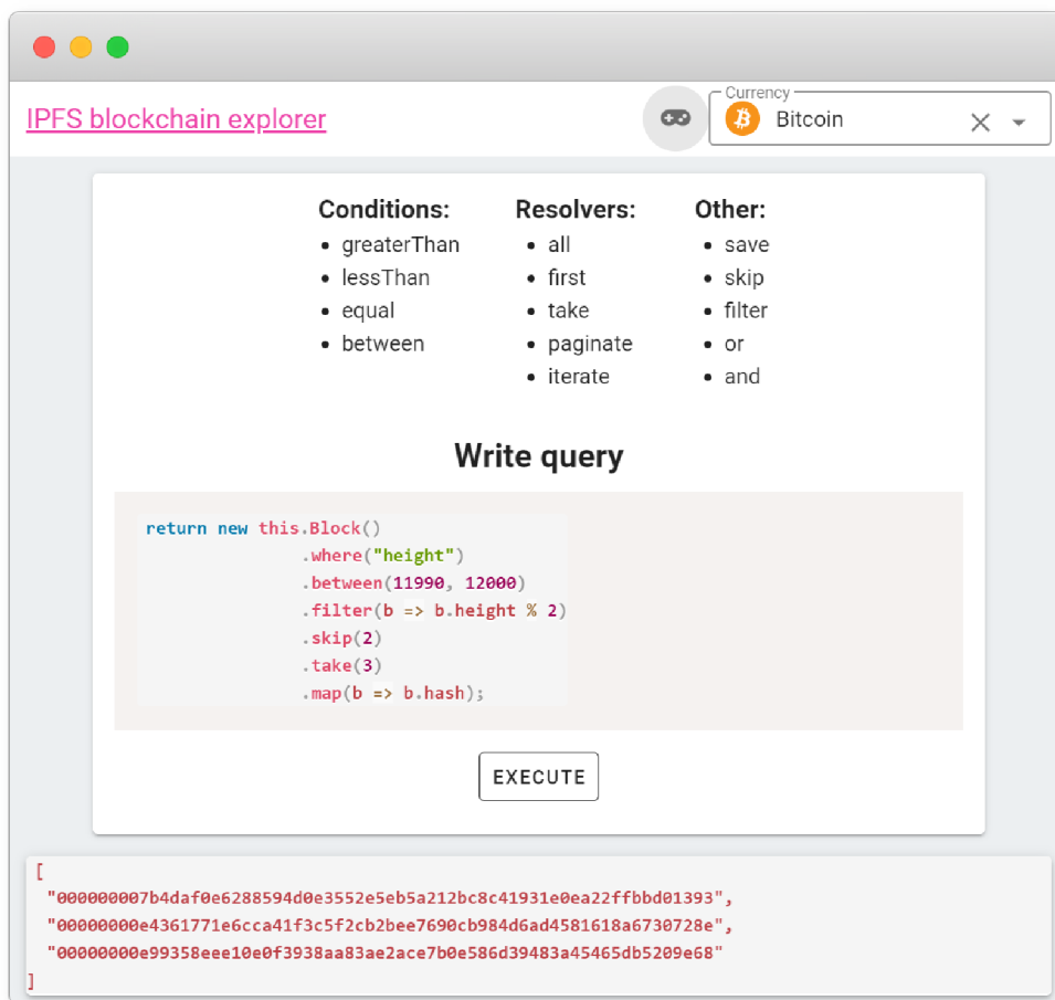
Figure 5.11: Playground view
