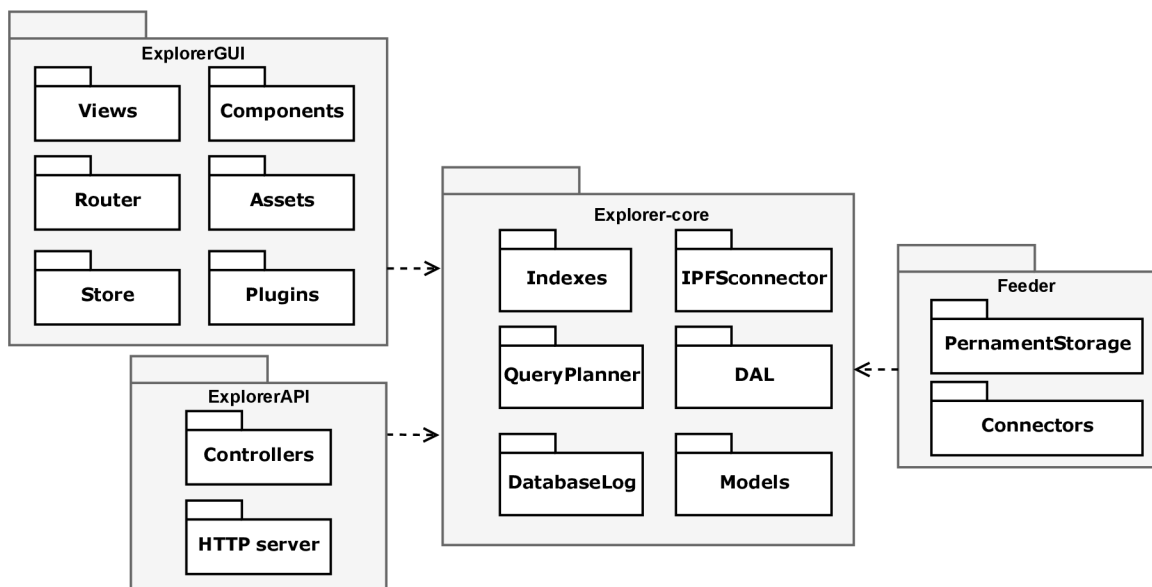
Figure 5.1: Platform architecture
