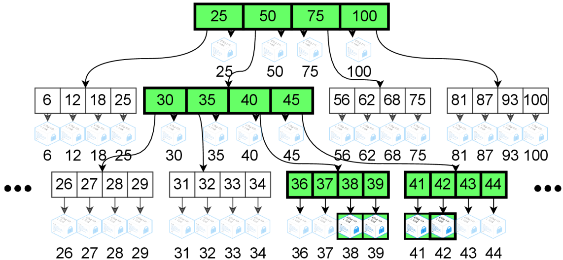
Figure 5.3: Data access for performing query that returns blocks that have a height between 38 and 42.
