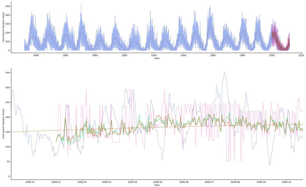
Figure 5.6: The picture above depicts sunspots (light blue curve), seasonal trend (dashed orange), prediction by DT (pink), RM (green] and grid search (red). The bottom picture is zoom in on the last part of the graph with tested outcome.
