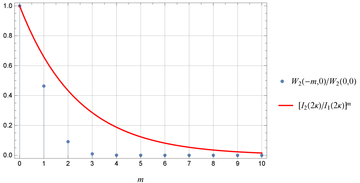
Figure 4.3: The quotient of the Wigner functions W_2^{[0,0]}(-m, 0)/W_2^{[0,0]}(0, 0) decreases at least as fast as [I_2(2\kappa)/I_1(2\kappa)]^m (here shown for \kappa = 2 ).
