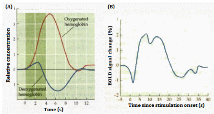
Fig. 3.1: (A) Changes in the concentrations of oxyhemoglobin and deoxyhemoglobin after neuronal activity and their impact on the BOLD signal (B) [7]
