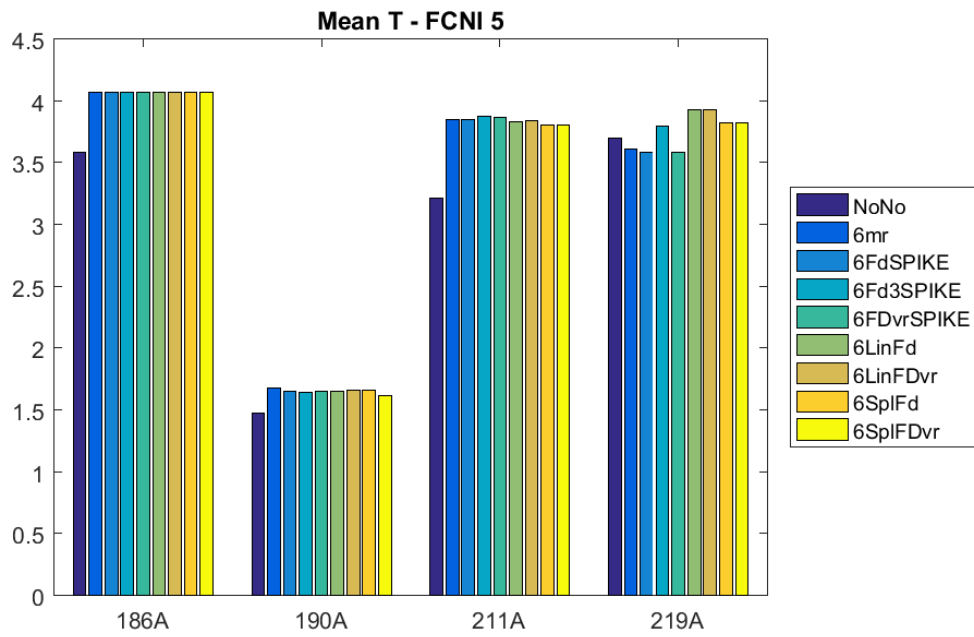
Fig. 11.11: Mean T-statistics for session FCNI5 across all subjects
