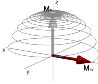
Fig. 2.3: Spiraling change (i.e. nutation) of a net magnetization after a 90^\circ radiofrequency pulse caused by diminishing M_z magnetization and growth of M_{xy} magnetization [8]
