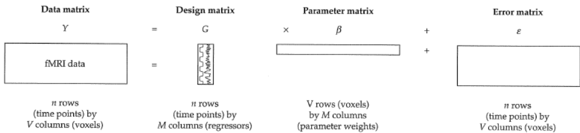
Fig. 6.2: General linear model tries to explain the original data ( Y ) by calculating parameter matrix \beta , which would provide the best fit for the design matrix ( G ) by minimizing the unexplained error \epsilon [7]
