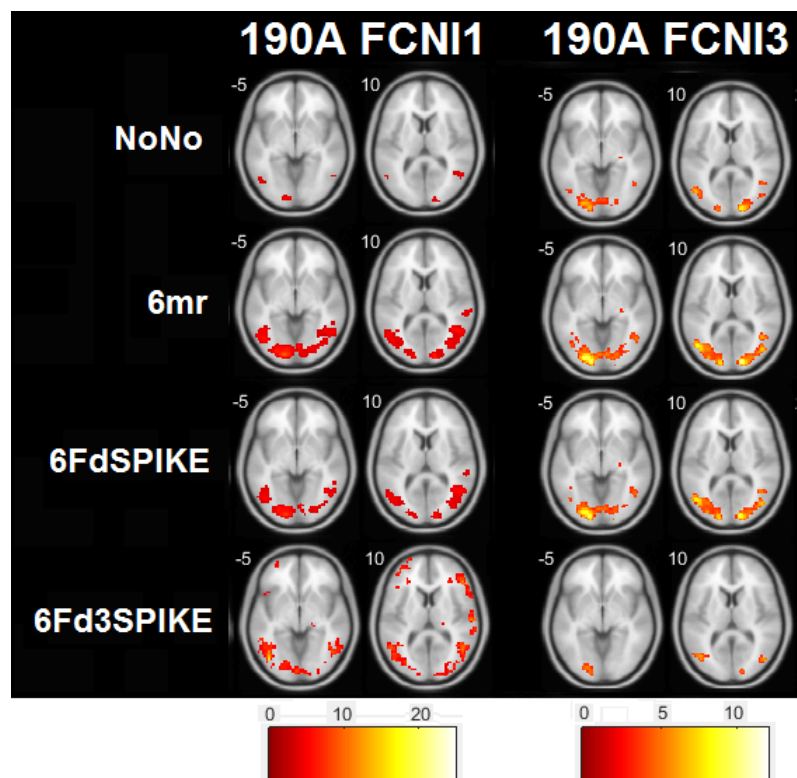
Fig. 11.12: Comparison of activation brain maps between session FCNI1 and FCNI3 for subject 190A
