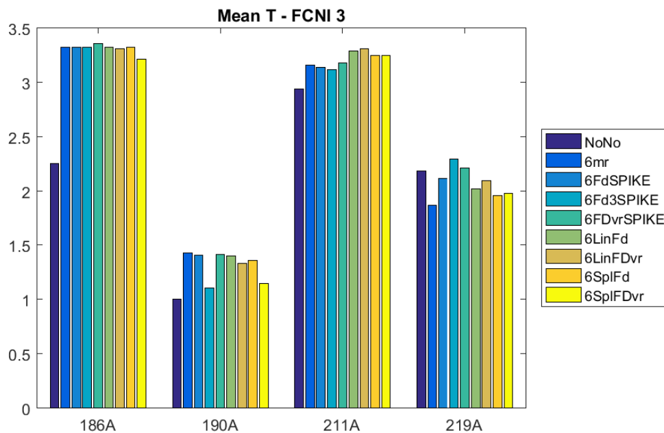
Fig. 11.10: Mean T-statistics for session FCNI3 across all subjects
