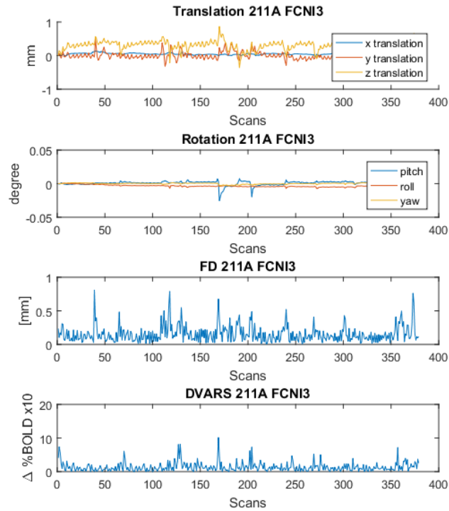
Fig. B.7: Motion prevalence in 211A FCN13
