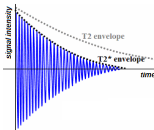
Fig. 2.4: Illustration of T_2 and T_2^* decay after applying a radiofrequency pulse, also known as free induction decay (FID) [6]
