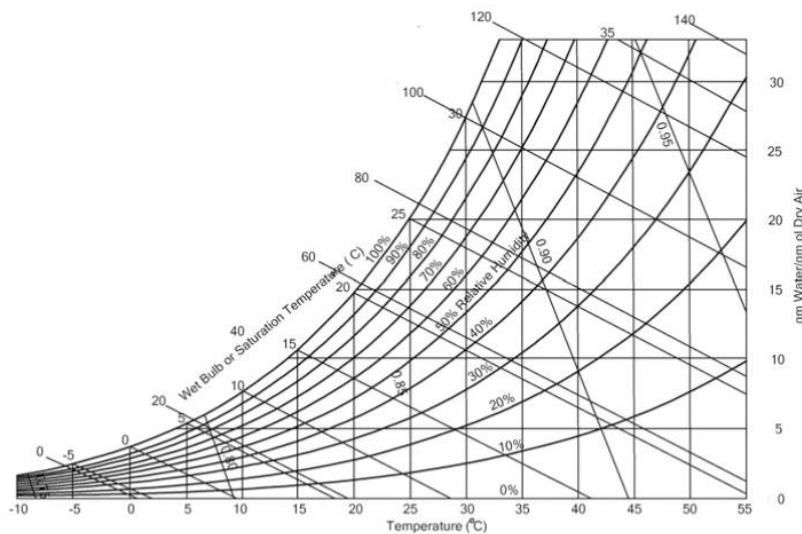
Figure 3: Psychrometric chart
