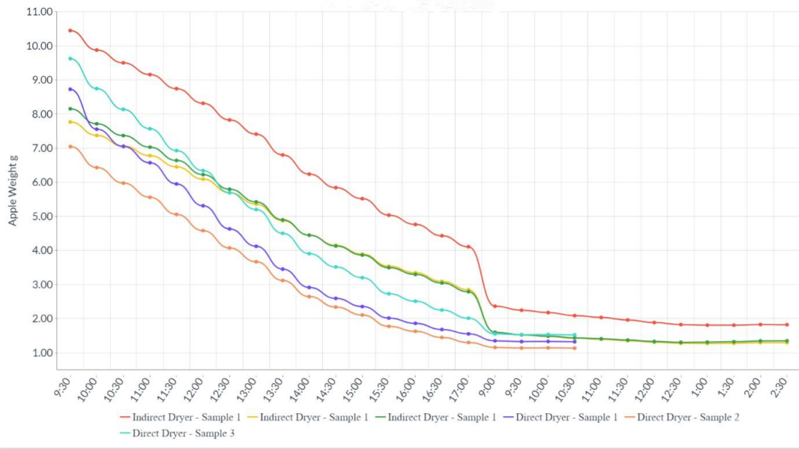
Figure 29: The first batch of apple drying - comparison between direct and indirect dryer (g)
