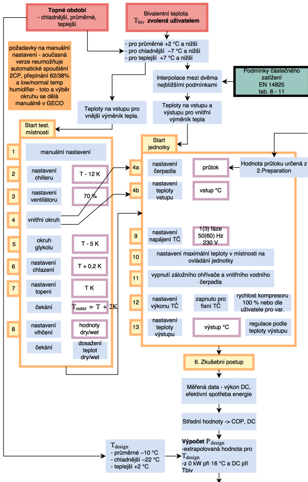
Obr. 10 Tbivalent
