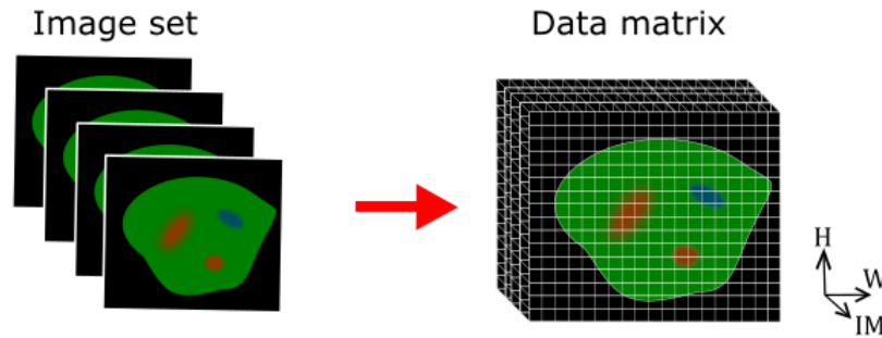
Fig. 17: Data representation
