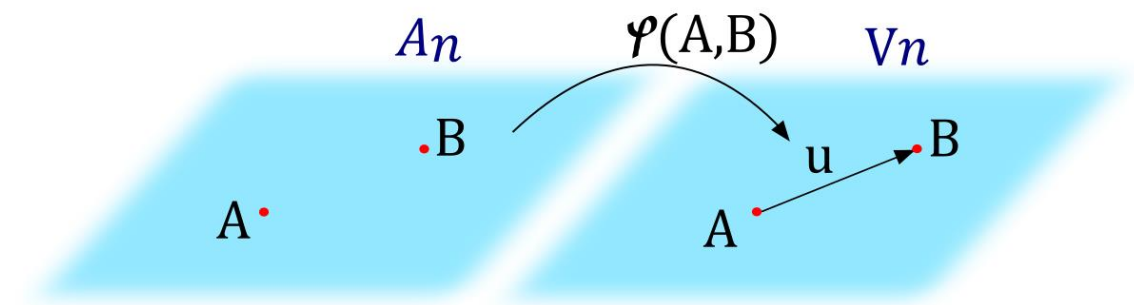
Fig. 5: Affine spaces
