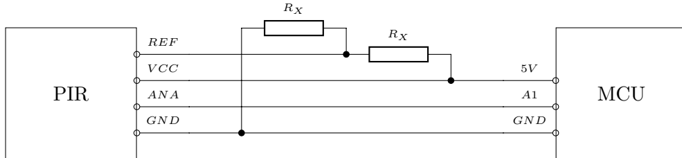
Figure 4.2: Connection of PIR and MCU.
