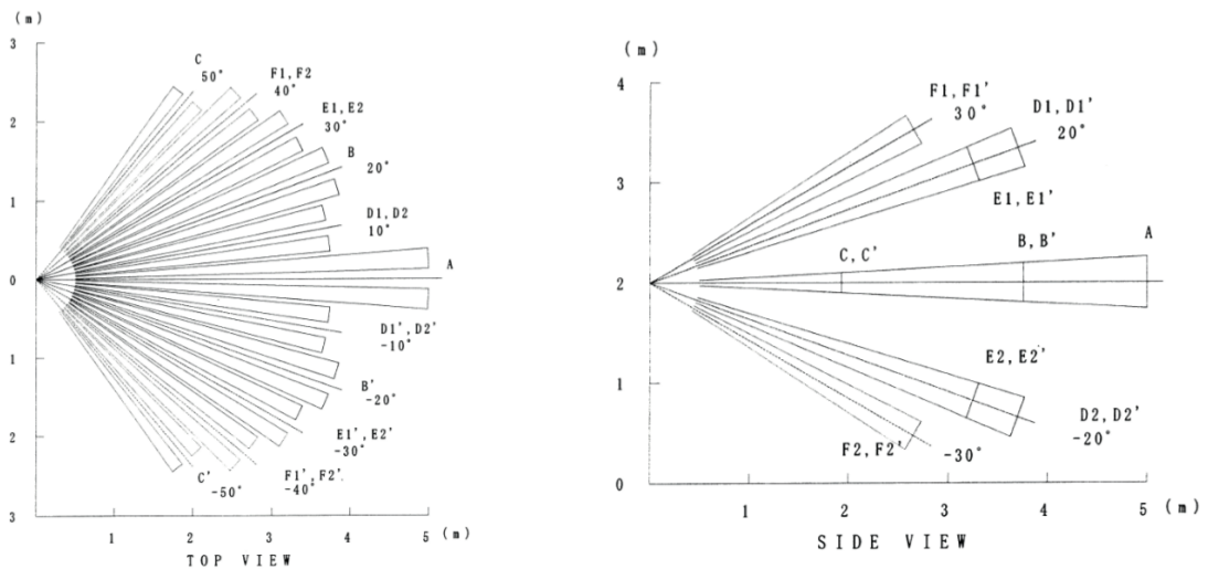
Figure 2.7: Sensing of PIR STD. [8]
