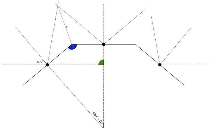
Figure 3.1: Geometry for three PIR sensors.
