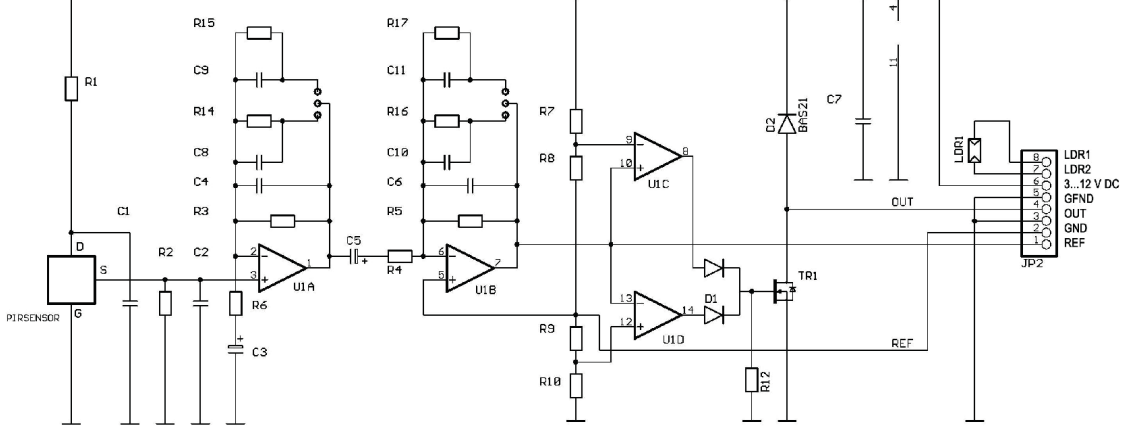
Figure 4.1: Scheme of PIR STD.[8]
