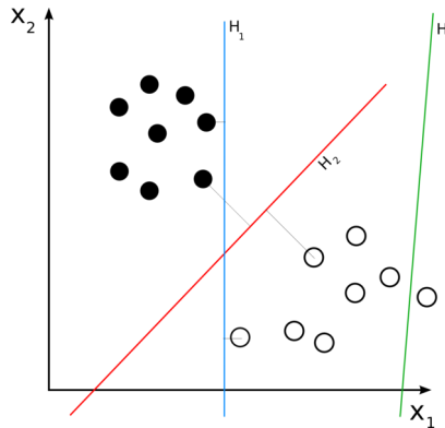
Figure 2.9: Linear classifier.[4]
