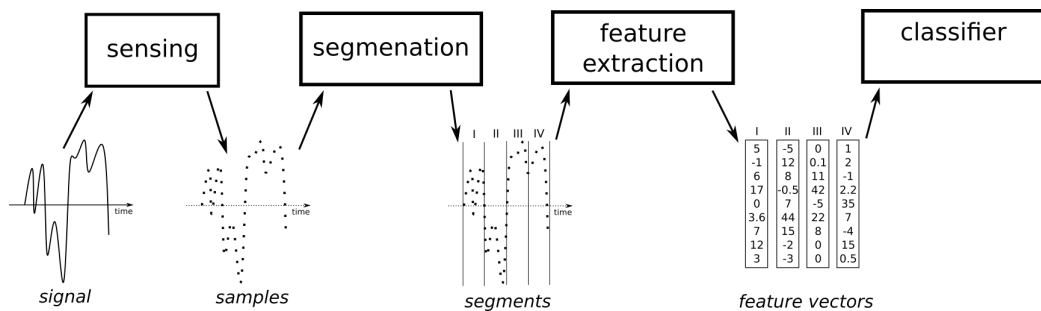
Figure 2.8: Preprocessing pipeline.
