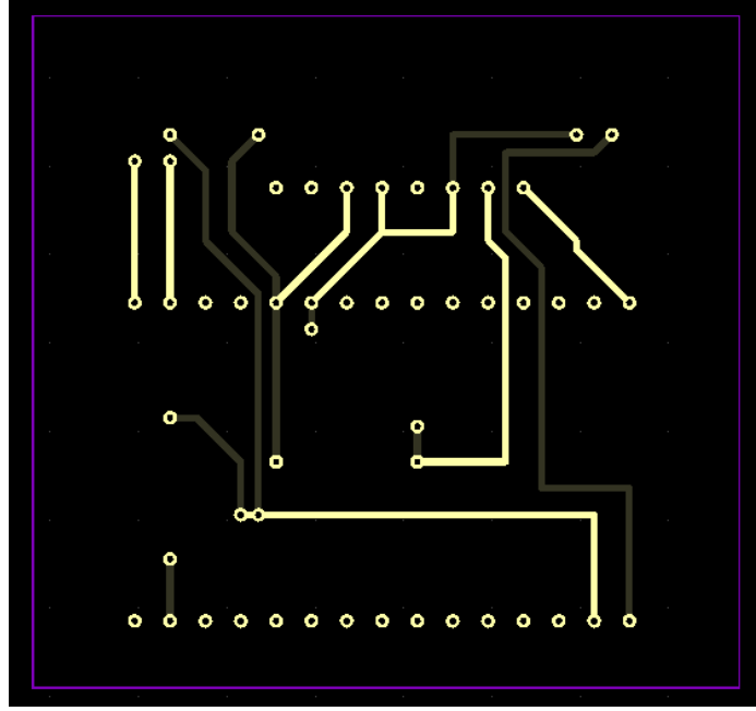
Figure 4.3: Circuit board.
