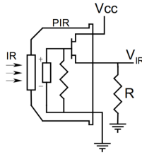
Figure 2.5: Single element pyroelectric detector.[7]
