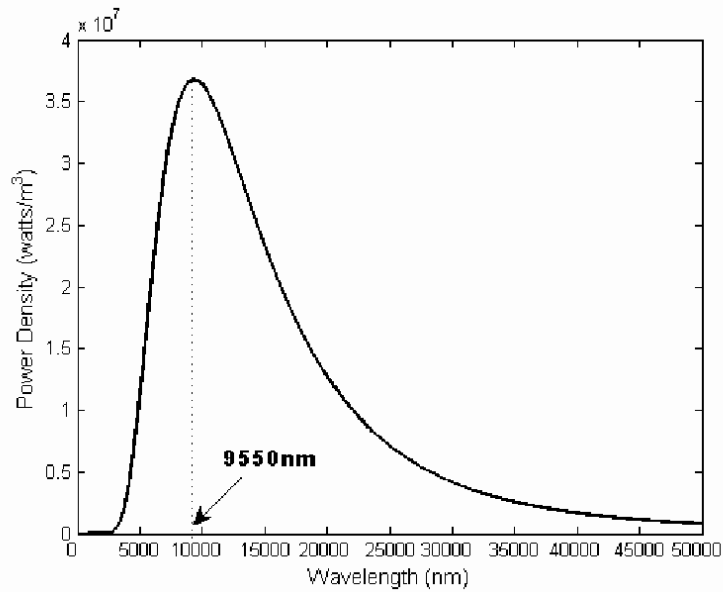
Figure 2.3: Human body radiation wavelength.[15]
