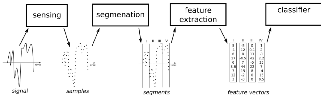
Figure 2.8: Preprocessing pipeline.
