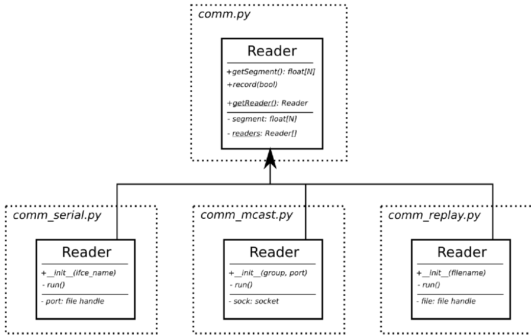
Figure 4.4: UML diagram of Reader classes.
