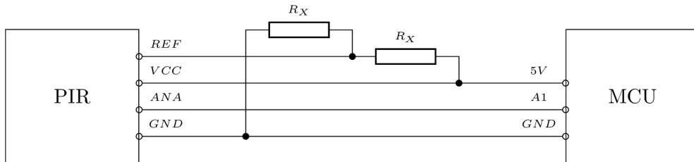
Figure 4.2: Connection of PIR and MCU.
