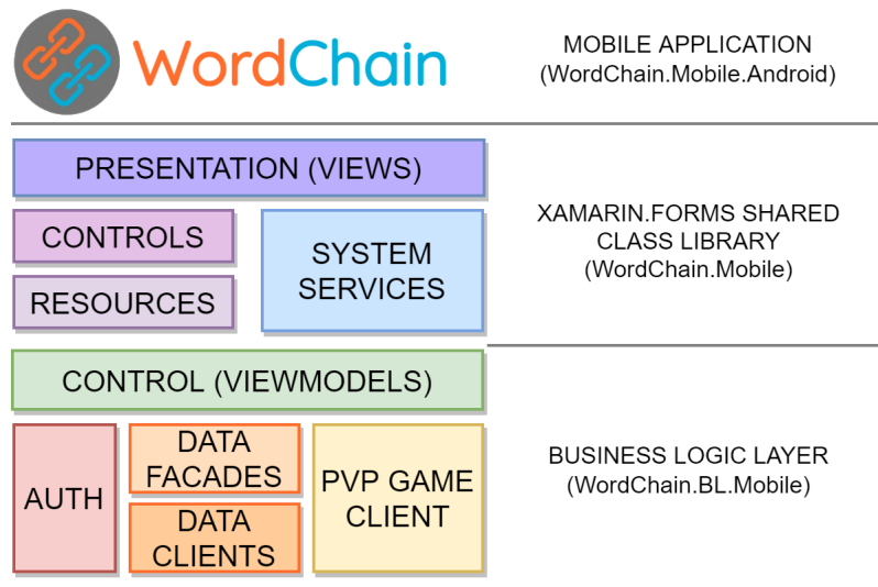
Figure 7.4: WordChain mobile application architecture
