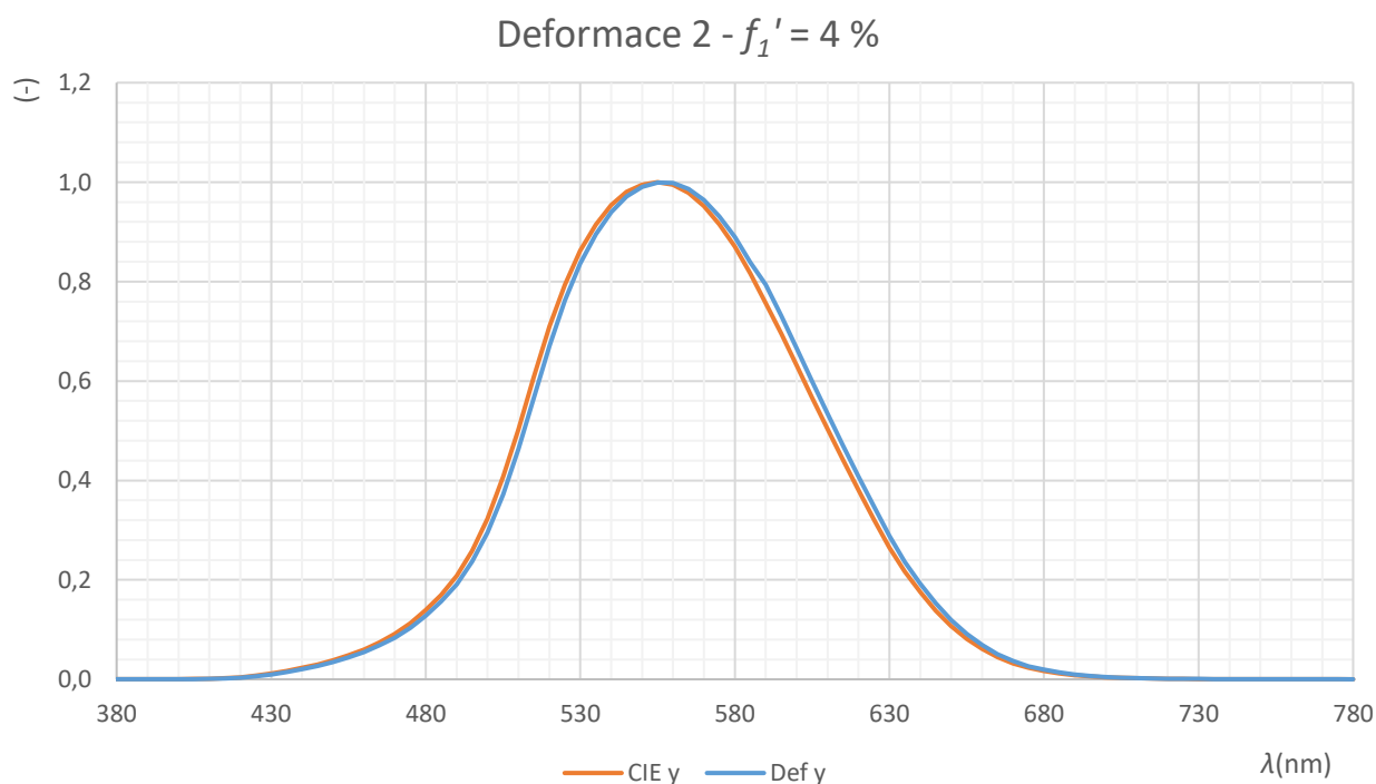
Obr. 38 Deformace 2 - f_l' = 4\%
