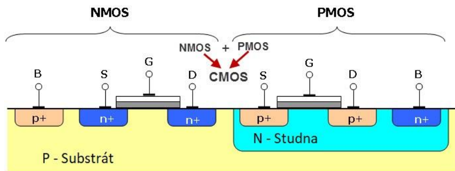
Obr. 19 CMOS technologie [12]
