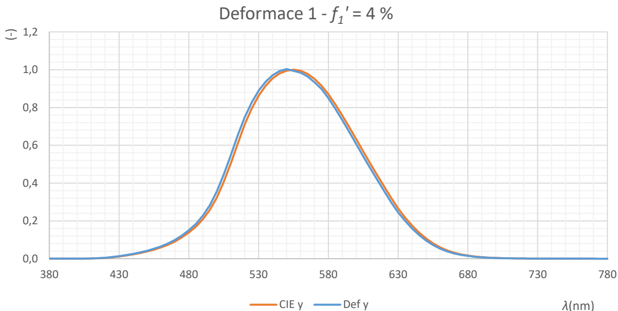
Obr. 37 Deformace 1 - f_l' = 4\%
