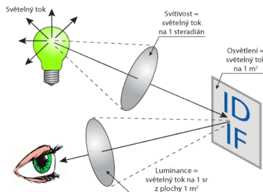
Obr. 1 Definice jasu [3]
