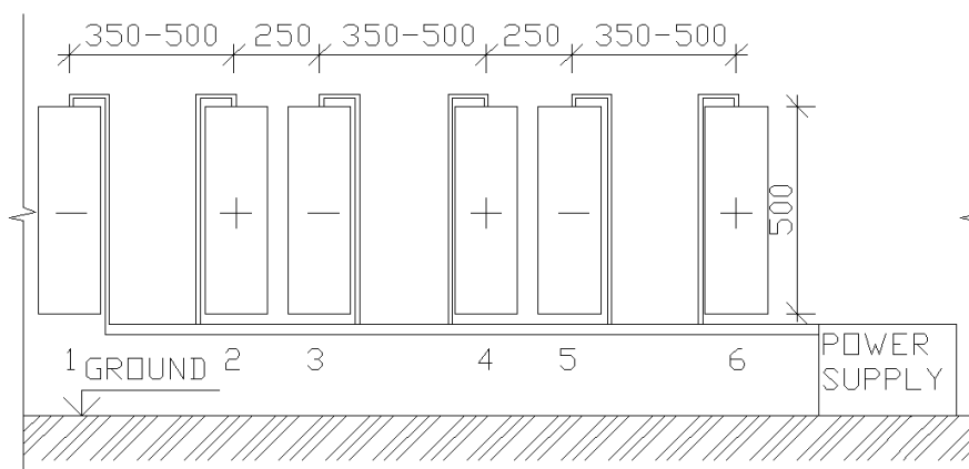
Fig. 69 The view on the electrode units and their recommended placement on the brick wall from the outer wall surface.
