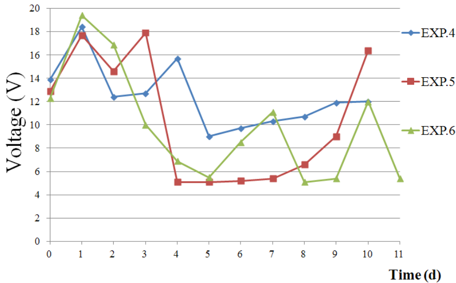
Fig. 41 The changes in the voltage during the experiments 4, 5 and 6 with the constant current 2 mA.
