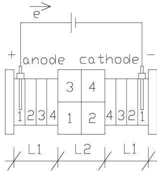
Fig. 16 The segmented parts, where the water contents and pH were measured. L1 – the clay poultice, L2 – half of the brick;
