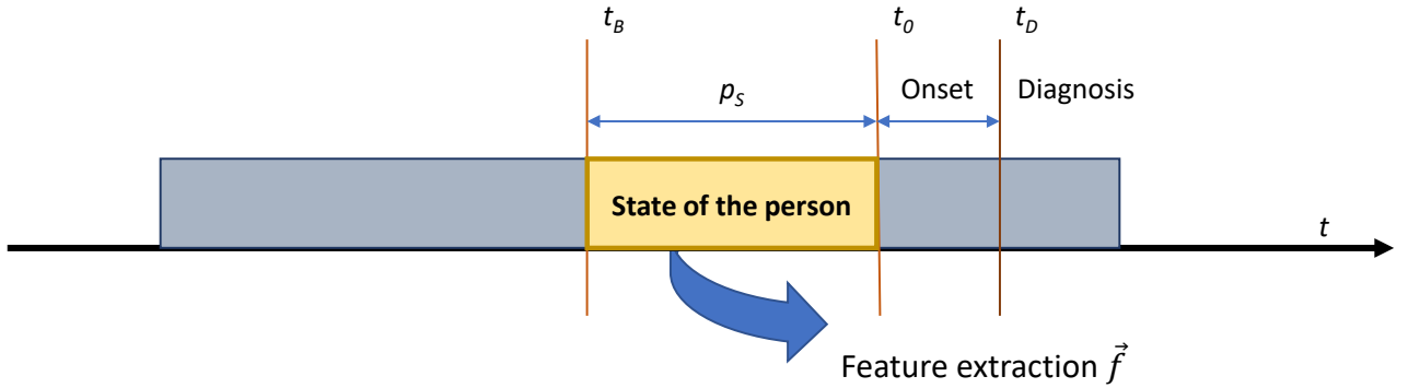
Fig. 3.2: Feature extraction.
