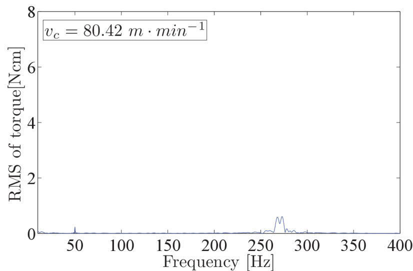
Figure 6.18: Zoomed spectral analysis of torque measurement data with proper grounding shown in Figure 6.16.
