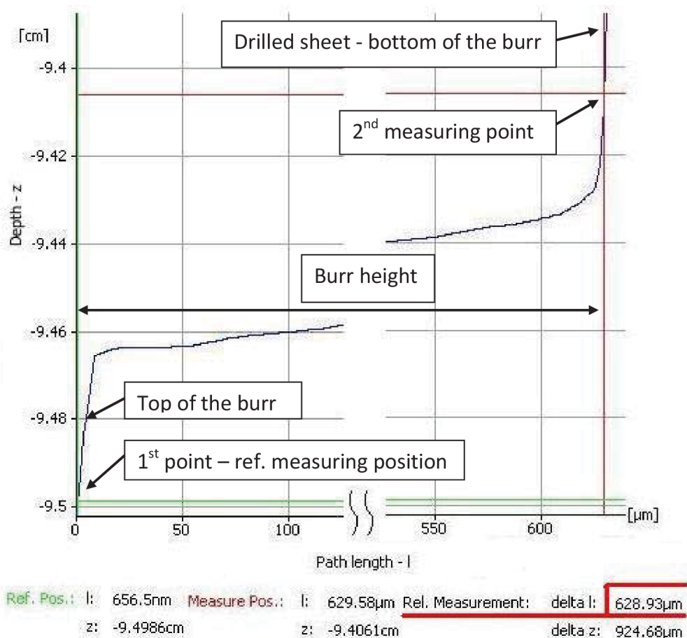
Figure 6.27: Profile measurement of the exit burr height in the MeX 5.1 software.
