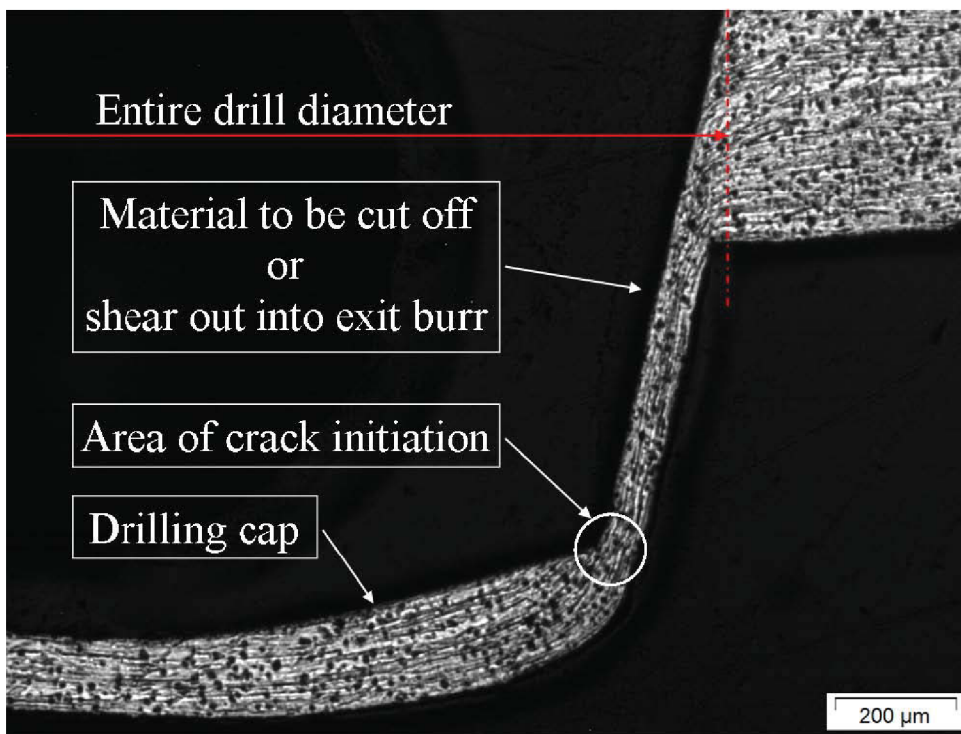
Figure 8.26: Etched cross-section view of exit burr, Drill A, zoomed on Figure 8.23.
