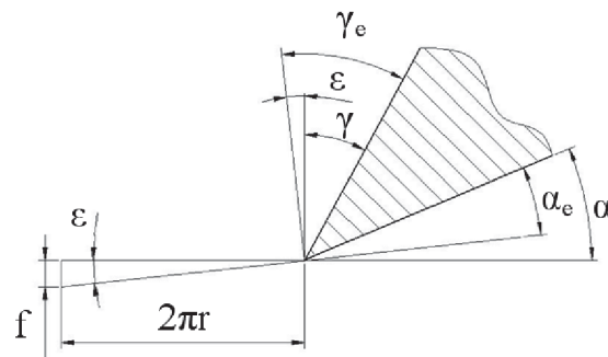
Figure 2.7: Feed angle during cutting.
