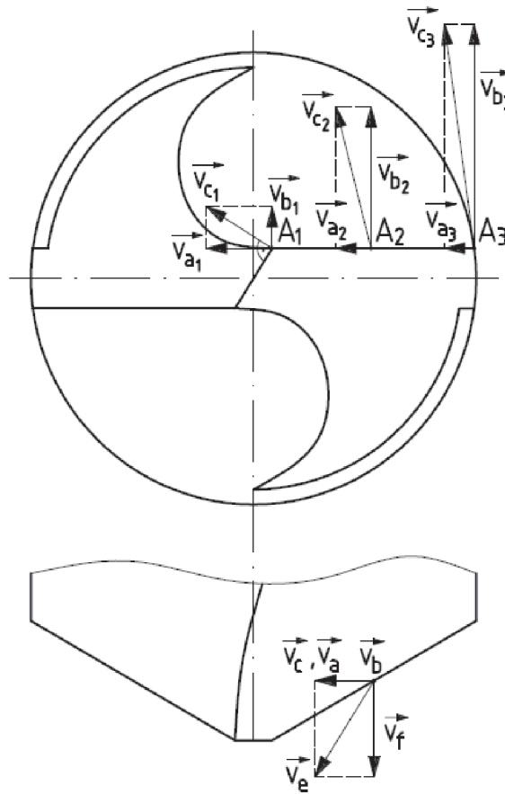
Figure 2.2: Directions of the primary and secondary movement when drilling with two-flute twist drill[9].
