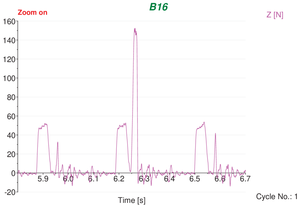
Figure 8.9: Peak in thrust force due to swarf clogged in drill flutes during drill retraction.
