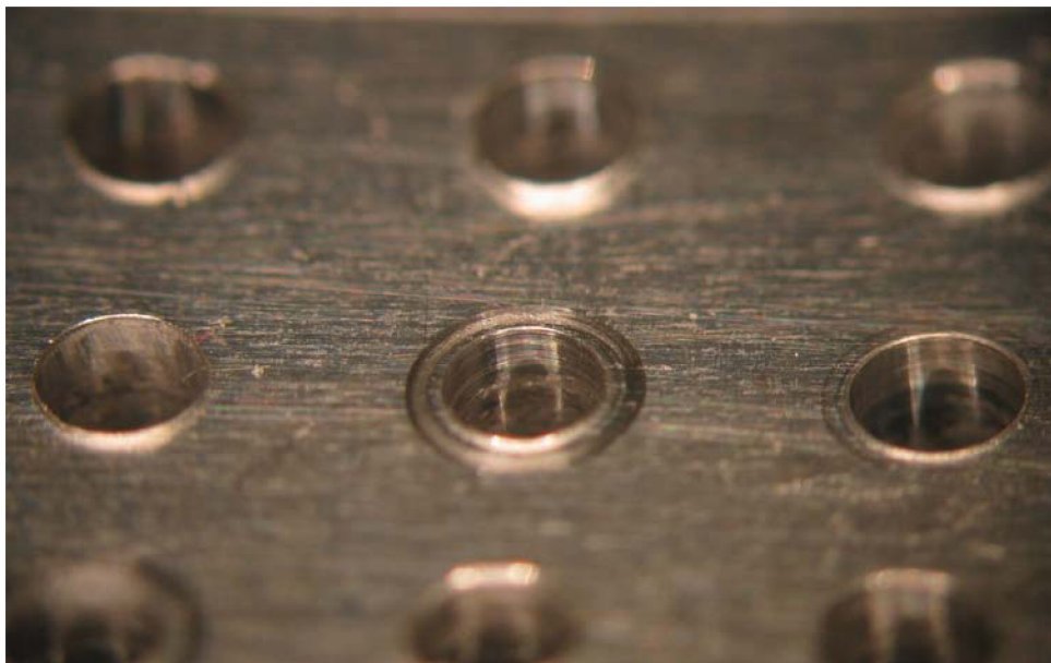
Figure 7.19: Scratched ring around the exit holes periphery.
