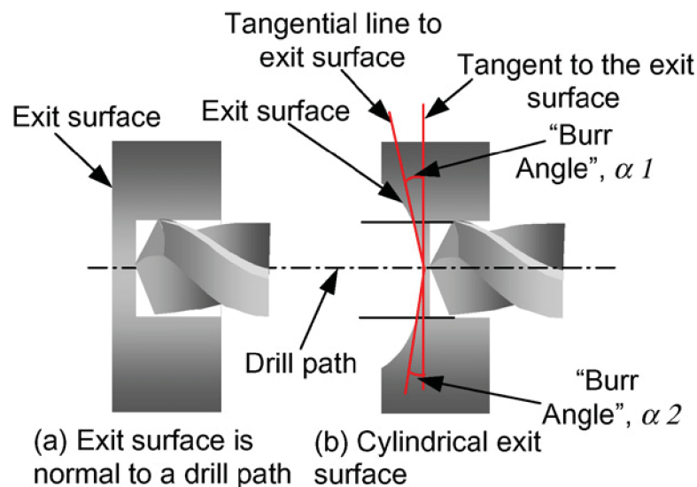
Figure 3.14: Burr formation when drilling intersection holes according to Min [39] depicted in [40].
