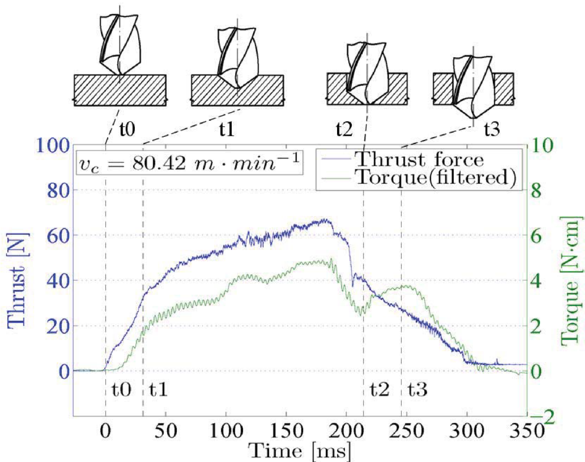
Figure 6.22: Description of force measurement plots with drill positions indicated.
