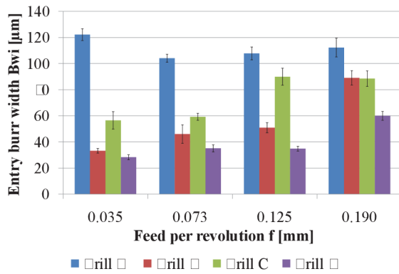
Figure 8.13: Comparison of entry burr widths resulting from four different drill geometries tested.
