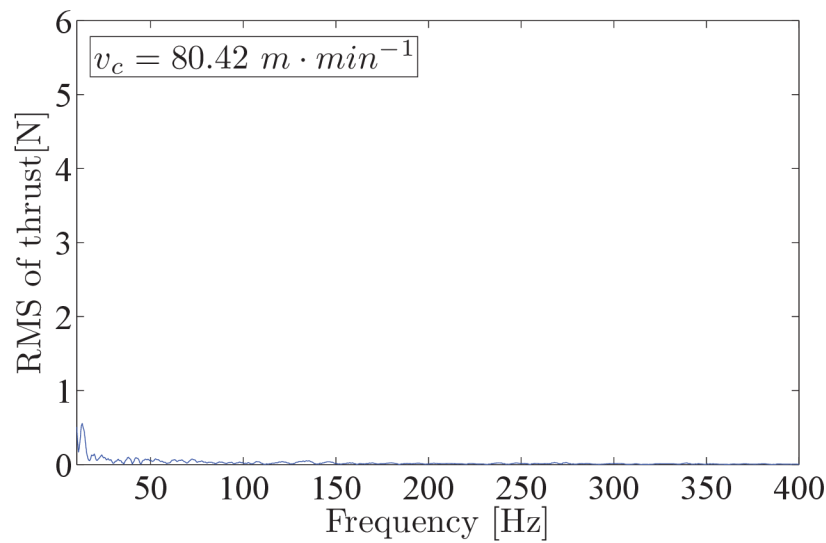
Figure 6.17: Zoomed spectral analysis of thrust measurement data with proper grounding shown in Figure 6.15.
