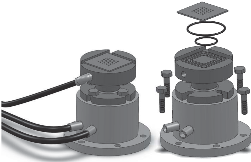
Figure 7.1: 3D model of the vacuum fixture constructed placed on the dynamometer.
