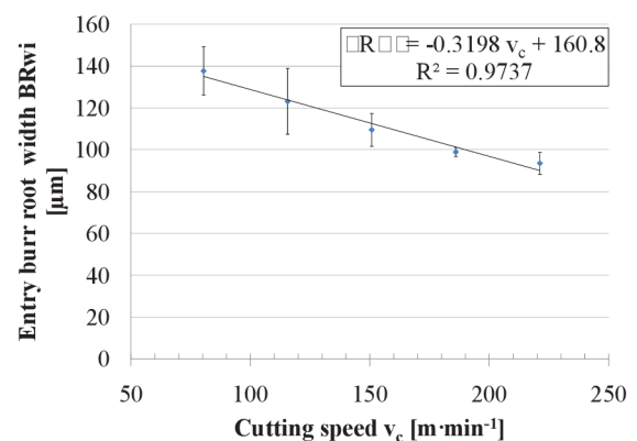
Figure 6.42: Influence of cutting speed on entry burr root width.
