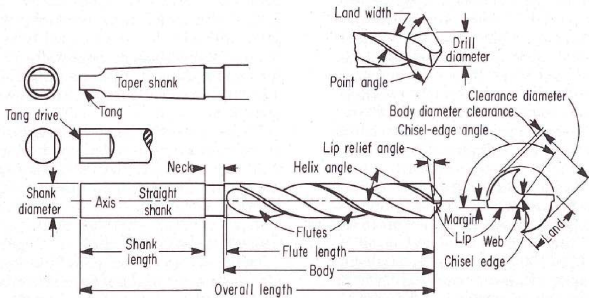
Figure 2.5: Drill nomenclature [10].
