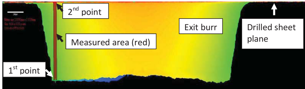
Figure 6.26: Evaluation of the exit burr height in MeX 5.1 software.
