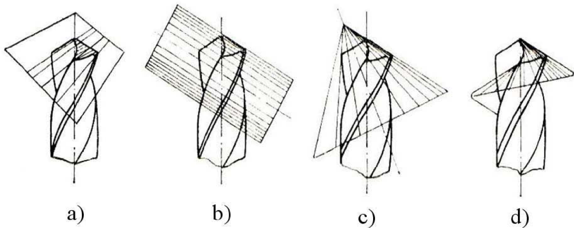
Figure 2.8: Point grinding methods for twist drill: a) Plain flank grinding, b) Cylindrical flank grinding, c) Conical flank grinding, d) Helical flank grinding [9].
