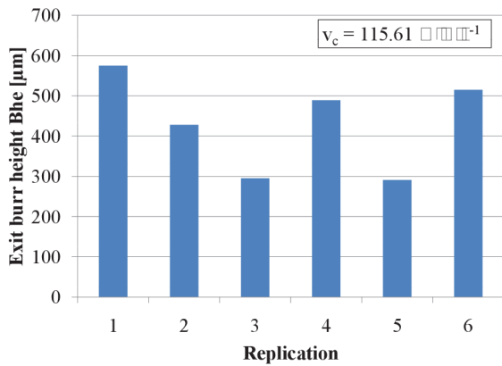
Figure 6.33: Burr heights variation when 6 replications of single drilling condition performed ( n = 23000 \text{ m} \cdot \text{min}^{-1} , f = 0.035 \text{ mm} ).
