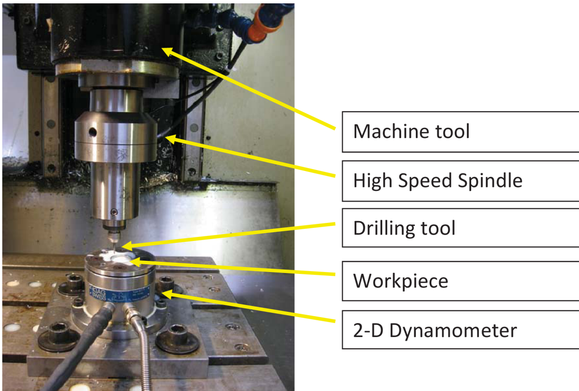
Figure 6.1: Experimental setup of preliminary drilling tests.
