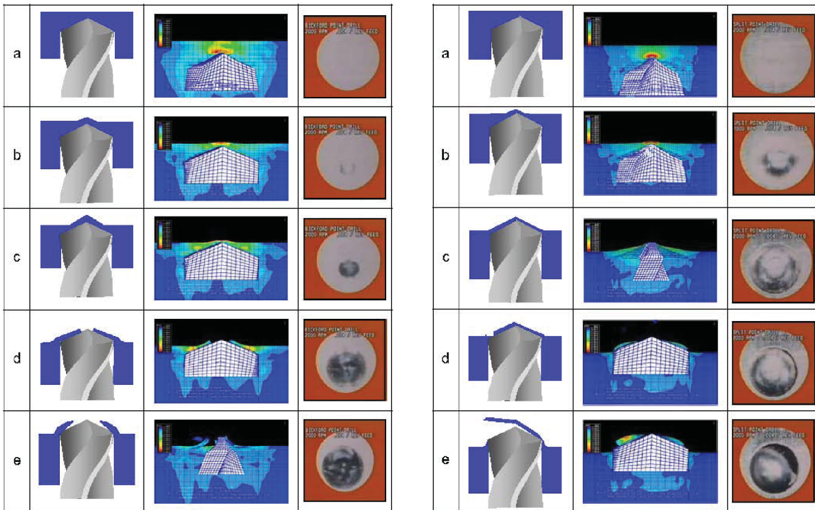
Figure 3.5: Burr formation mechanism of a crown burr — left picture, an uniform burr with a drilling cap — right picture [21].
