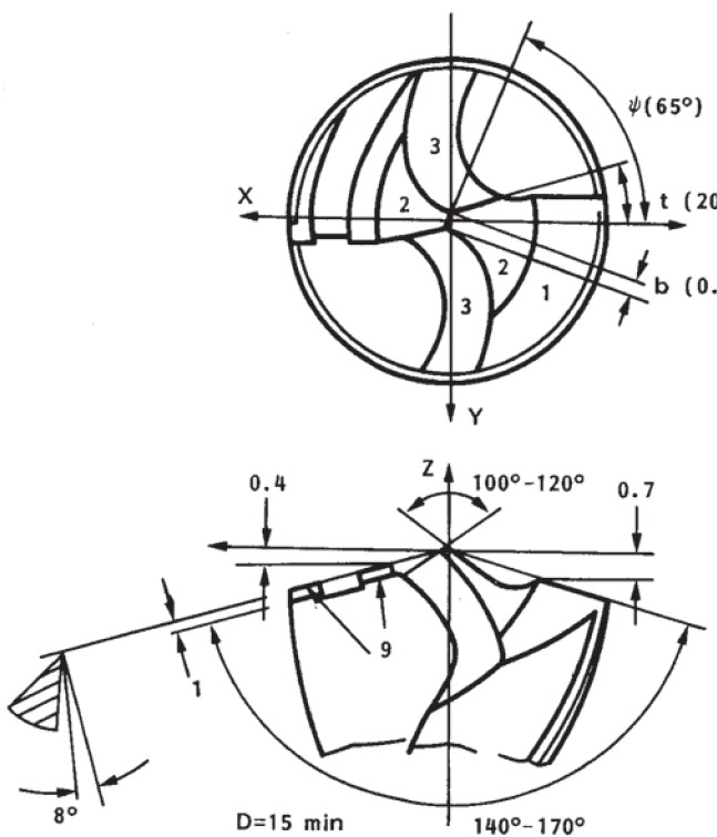
Figure 2.20: MFD for drilling aluminum alloys [11].
