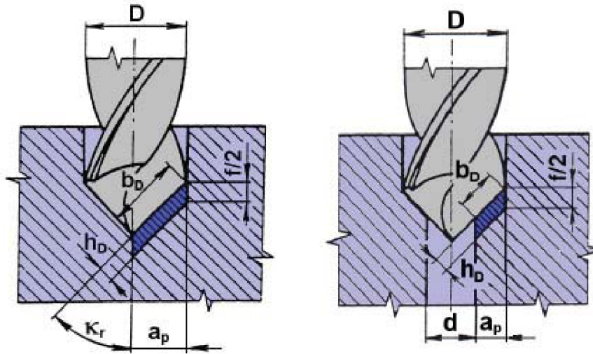
Figure 2.3: Geometrical elements of the undeformed chip: in plain drilling (left), in secondary drilling (right)[9].
