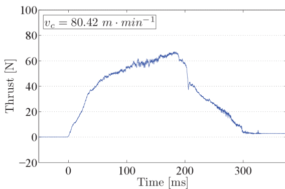
Figure 6.15: Thrust force measurement with proper grounding ( n = 16000 \text{ min}^{-1} , f = 0.035 \text{ mm} ).
