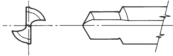
Figure 2.22: Step drill geometry [6].
