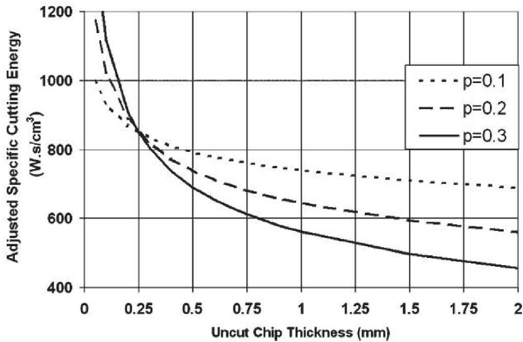
Figure 3.10: Adjusted specific cutting energy vs. uncut chip thickness [35] depicted in [33]
