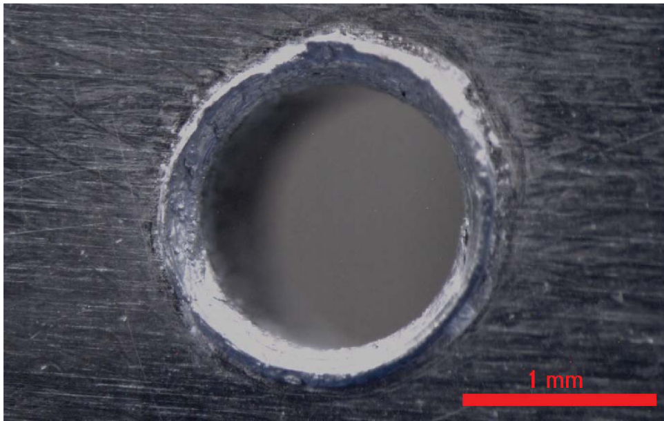
Figure 6.53: Problem at the hole entry caused by drill wandering on the workpiece surface when drilling began.
