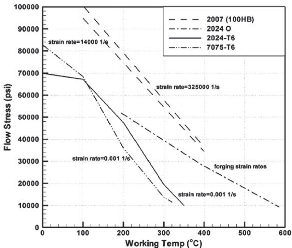
Figure 3.12: Flow stress vs. temperature (various references cited in [33]) 1
