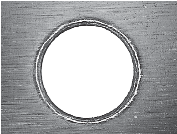
Figure 6.51: Ordinary hole entry with burr formed.
