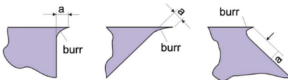
Figure 3.6: Burr geometry according to ISO 13715 [?], picture from [3].
