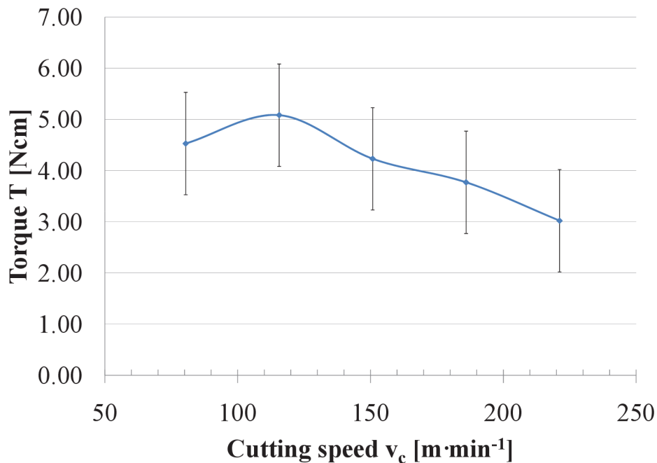
Figure 6.31: Influence of cutting speed on drilling torque.
