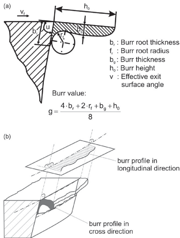
Figure 3.7: Measurement values of a burr according to Schäfer [3].
