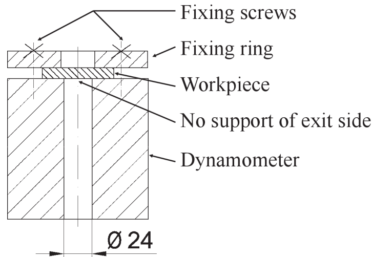
Figure 6.3: Schematic of clamping system used during the preliminary test.
