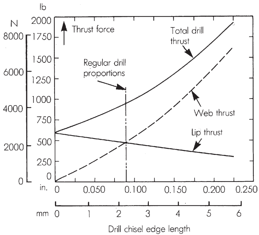
Figure 2.12: Effect of chisel edge length on thrust force [6].
