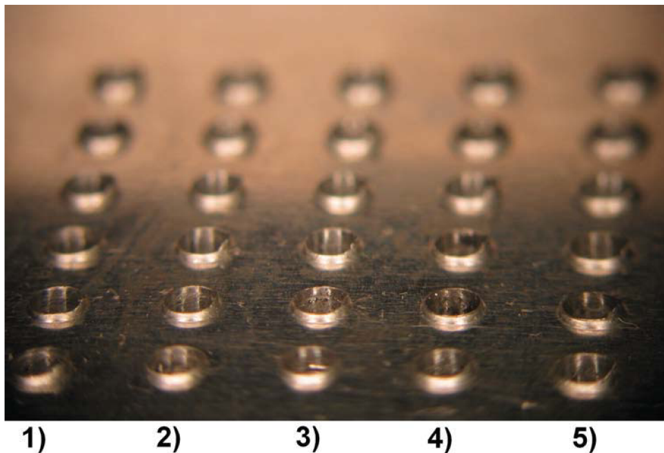
Figure 7.8: Photograph of exit burrs resulting from the 2nd clamping investigation setting (see Figure 7.7) with indication of used setting (an investigation of feed per revolution on burr formation).
