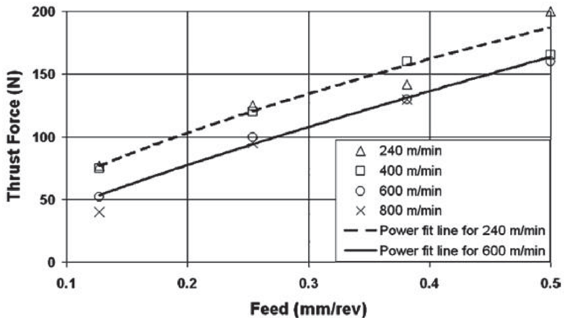
Figure 3.11: Thrust force vs. feed at different speeds [33] based on [36] data.
