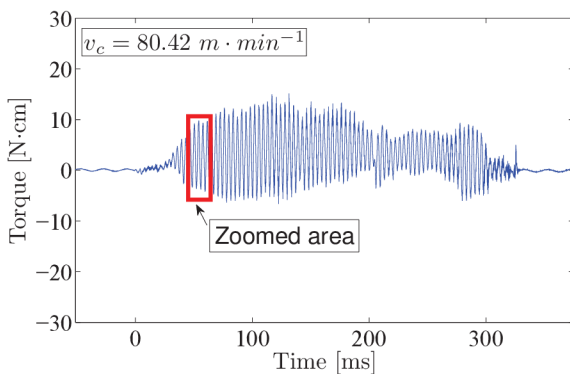
Figure 6.19: Torque measurement from Fig. 6.16 data with depicted zoomed area on fluctuation.
