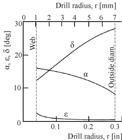
Figure 2.6: Variation of helix angle \delta , clearance angle \alpha , and feed angle \varepsilon , across the cutting edge of a representative 14.3 mm diameter drill. Helix angle, 28°; clearance angle, 8°; point angle 118°; chisel edge angle, 120°; web thickness, 2.03 mm, feed rate, 0.23 mm [10].
