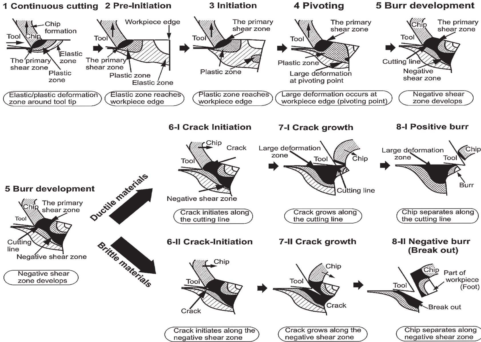
Figure 3.2: Schematic of burr formation [15] depicted in [3].
