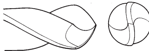
Figure 2.18: Rounded-edge point which has lips and margins blended by smooth curves [6].
