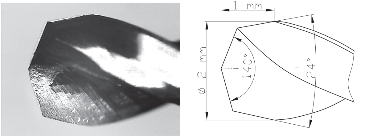
Figure 8.1: Profile of double cone point Drill A.
