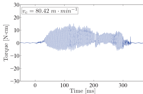
Figure 6.16: Torque measurement data with proper grounding ( n = 16000 \text{ min}^{-1} , f = 0.035 \text{ mm} ).
