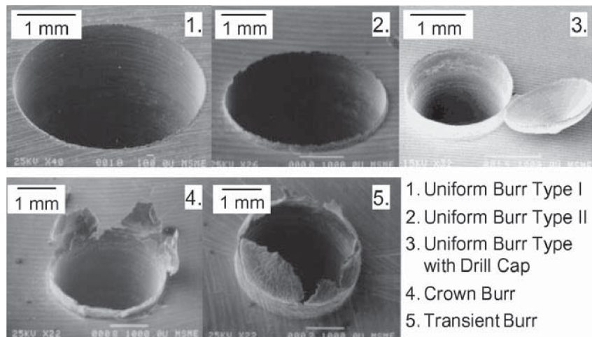
Figure 3.4: Typical drilling burr types by CODEF [19].
