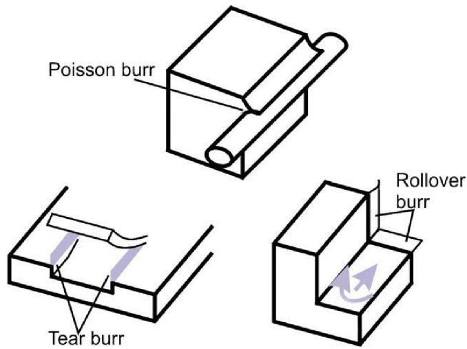
Figure 3.3: Schematic of poisson, tear and rollover burr [16].
