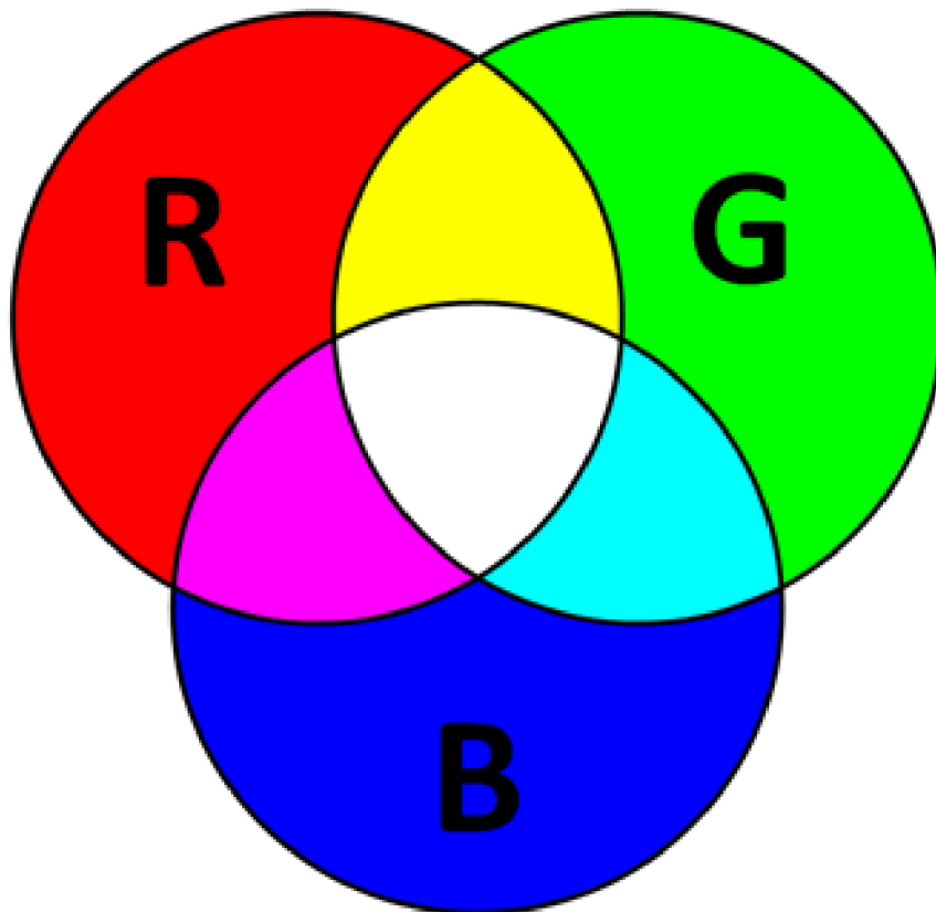
Obr. 1.2: Model RGB
