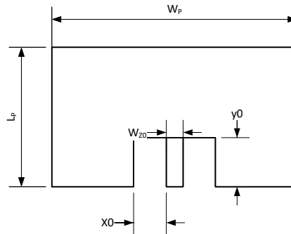
Fig. 1.7: Inset-fed patch
