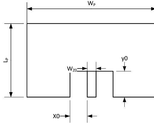
Fig. 2.1: Inset-fed patch
