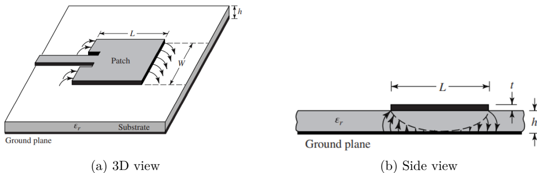
Fig. 1.2: Patch antenna [1]
