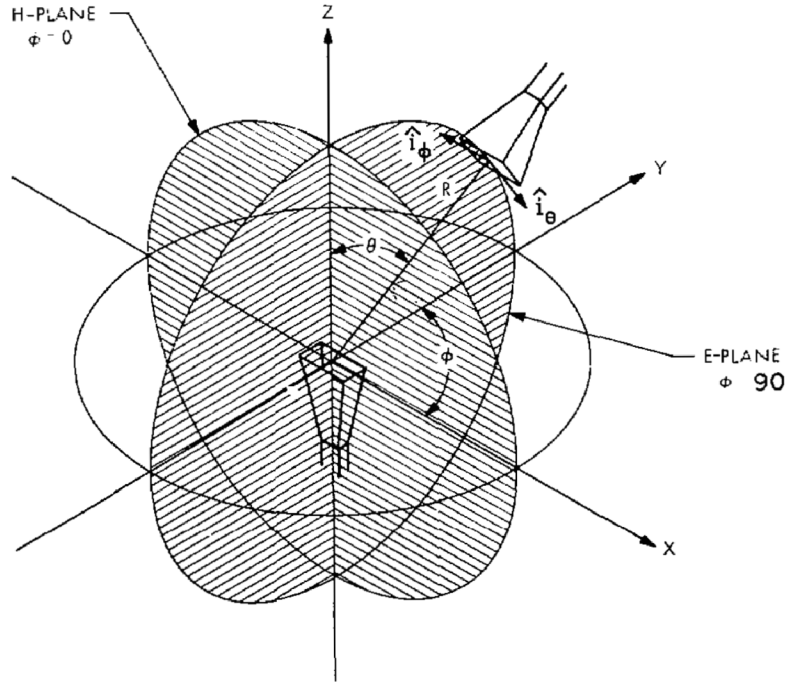
Fig. 1.13: Antenna polarisation measurement[2]
