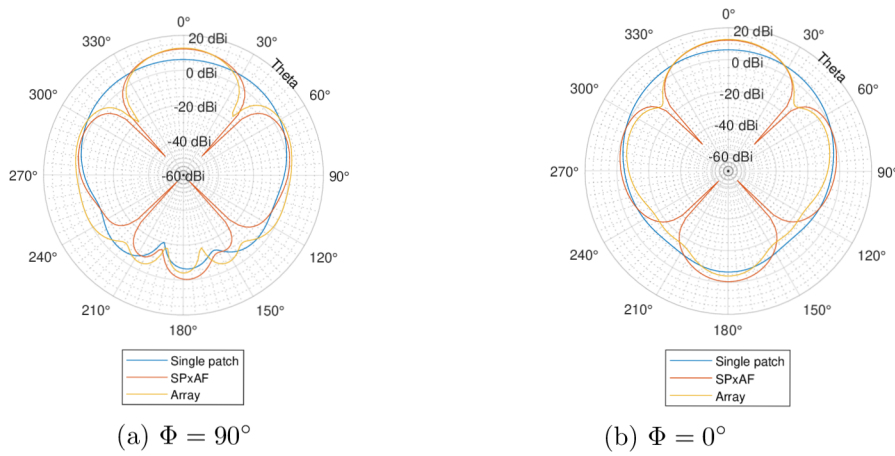
Fig. 3.15: Total realized gain of the proximity-fed antenna on RO4350 substrate
