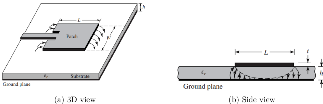
Fig. 1.2: Patch antenna [1]
