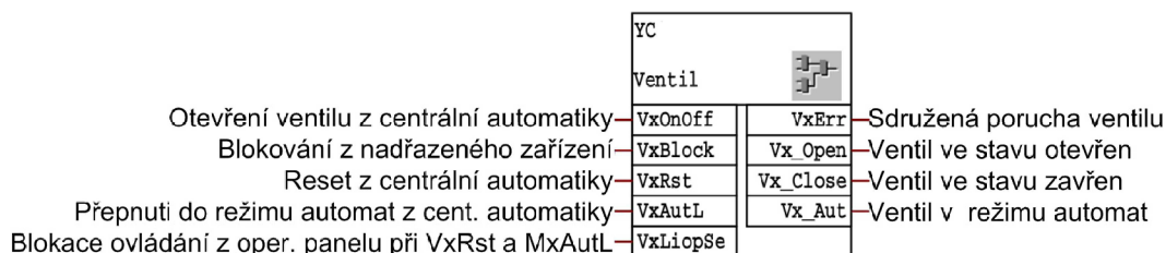
Obr. 8.3: CFC ventilu
