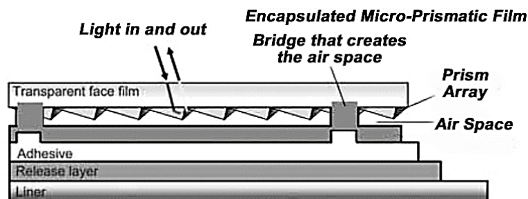
Fig. 17 Sectional view of a structure of encapsulated unmetalled microprismatic sheeting. Source: retrieved from Stein et al. (1989)
