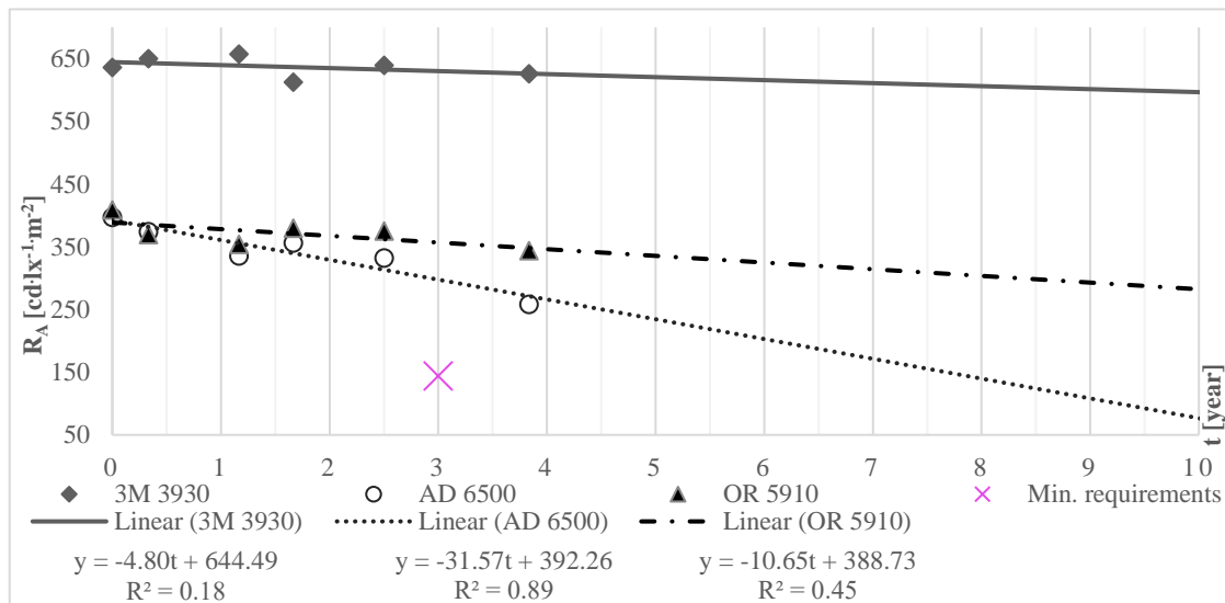
Fig. 44 Degradation trends of R_A ( \text{cd}\cdot\text{lx}^{-1}\cdot\text{m}^{-2} , \alpha = 0.33^\circ , \beta_1 = 5^\circ ) for white microprism. RA2 sheeting exposed to accel. natural weathering. Source: Author's work
