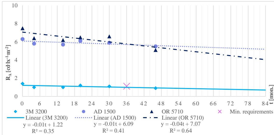
Fig. 43 Degradation trends of R_A ( \text{cd}\cdot\text{lx}^{-1}\cdot\text{m}^{-2} , \alpha = 0.33^\circ , \beta_1 = 5^\circ ) for blue glass bead sheeting Class RA1 exposed to accelerated natural weathering. Source: Author's work
