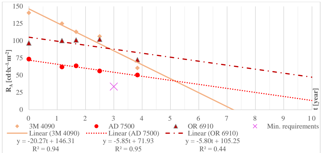
Fig. 48 Degradation trends of R_A ( \text{cd}\cdot\text{lx}^{-1}\cdot\text{m}^{-2} , \alpha = 0.33^\circ , \beta_1 = 5^\circ ) for red microprismatic sheeting Class RA3 exposed to accelerated natural weathering. Source: Author's work
