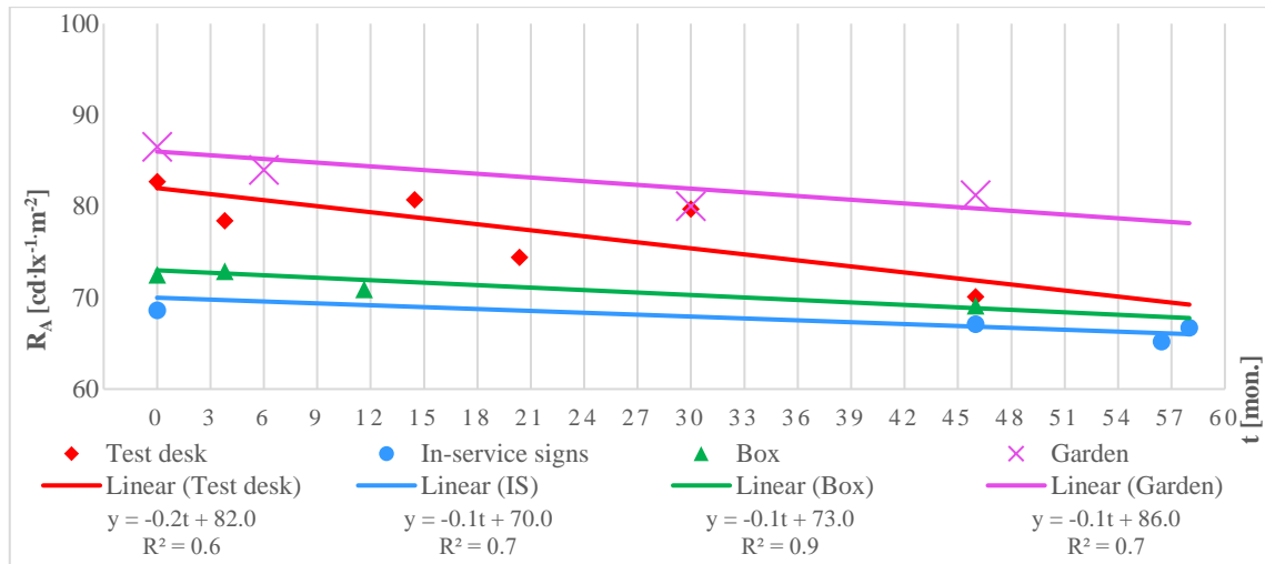
Fig. 58 The degradation trendlines of R_A ( \text{cd}\cdot\text{lx}^{-1}\cdot\text{m}^{-2} , \alpha = 0.33^\circ , \beta_1 = 5^\circ ) for one white glass-bead Class RA1 sample from four study locations. Source: Author's work
