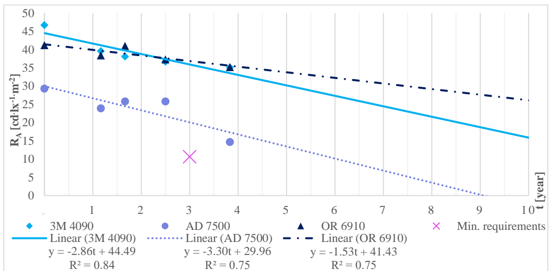
Fig. 49 Degradation trends of R_A ( \text{cd}\cdot\text{lx}^{-1}\cdot\text{m}^{-2} , \alpha = 0.33^\circ , \beta_1 = 5^\circ ) for blue microprismatic sheeting Class RA3 exposed to accelerated natural weathering. Source: Author's work
