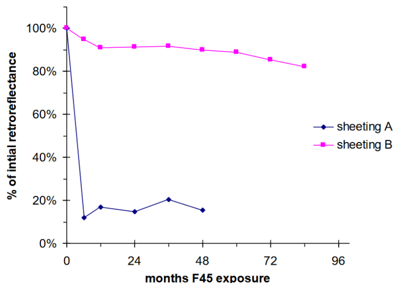
Fig. 20 Dramatic durability difference between two Type III sheetings after accelerated natural exposure in Florida. Source: retrieved from Ketola (1999)
