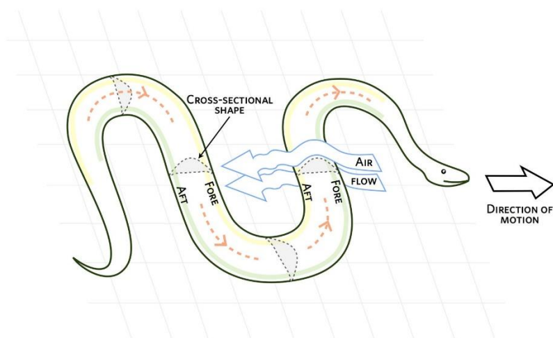
Obr. 3: Lietajúci had [5]
