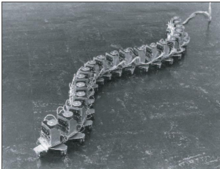
Obr. 13: Robot ACM-III [8]
