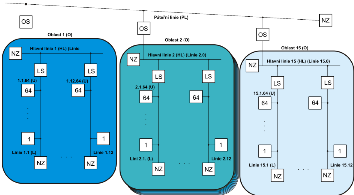
Obr. 3-5 Topologie [11]
