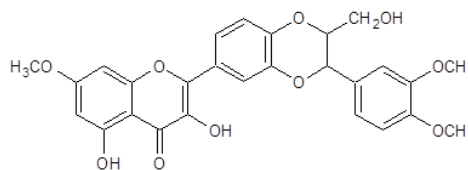
7,20-di- O -methyl-2,3-dehydrosilybin
