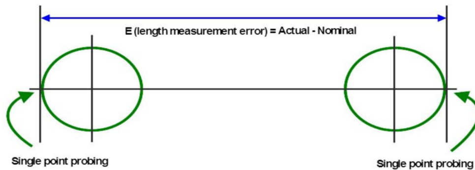
Figure 22 Length measurement error [19]
