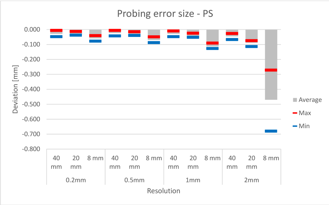
Graph 3 Probing error Size-Resolution
