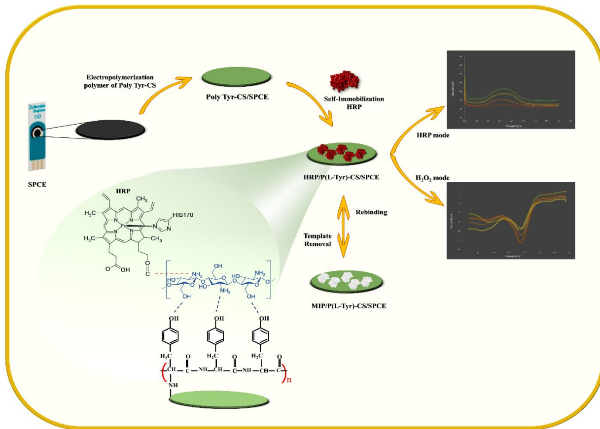
Scheme. 4.4 | The preparation process of MIP/poly(Tyr)-CS/SPCE biosensor.
