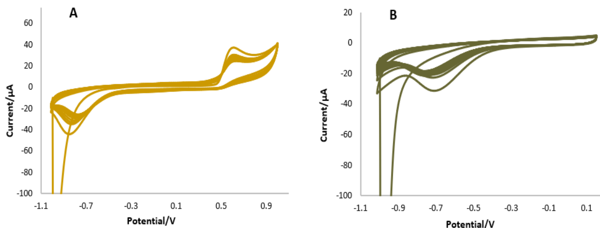
Fig. 4.16 | A) CVs of poly(Tyr) on the surface of SPCE in the presence of 0.1 M PBS (pH=7.4) containing 27 mM L -Tyr at scan rate of 100 \text{mV s}^{-1} . Number of cycles is 10. B) CVs of CS on the surface of SPCE in the presence of 0.1 M HCl containing 2 mg/mL CS at scan rate of 100 \text{mV s}^{-1} . Number of cycles is 20.
