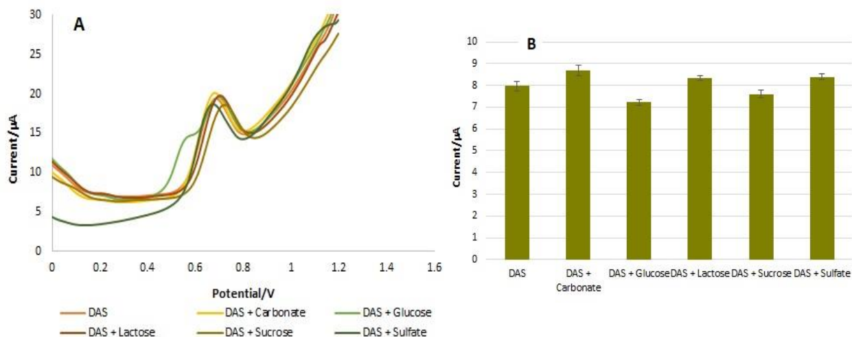
Fig. 4.6 | (A) Interference effect of lactose, sucrose, glucose, \text{SO}_4^{2-} , and \text{CO}_3^{2-} on determination of DAS by SWV method on SWCNT-COOH-SPCEs in supporting electrolyte Britton-Robinson buffer pH 5.0. (B) Histogram of interference effect.
