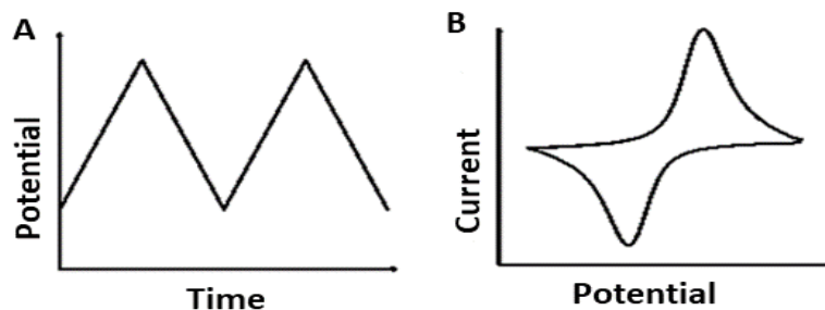
Fig. 2.3 | Cyclic voltammetric technique. (A) The potential cycling waveform. (B) An example of a typical cyclic voltammogram for a reversible redox process.
