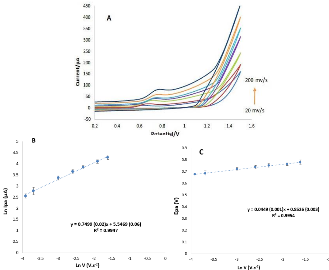
Fig. 4.5 | The effect of scan rate (A) CV of 100 μM dasatinib at SWCN1-modified SPCE; Britton-Robinson buffer pH 5.0; scan rates 20, 25, 50, 75, 100, 150, 200 mV.s -1 . (B) The plot of ln I pa (Napierian logarithm of oxidation peak currents) versus ln V (Napierian logarithm of scan rates). (C) Dependency of oxidation E pa (peak potentials) versus ln V.
