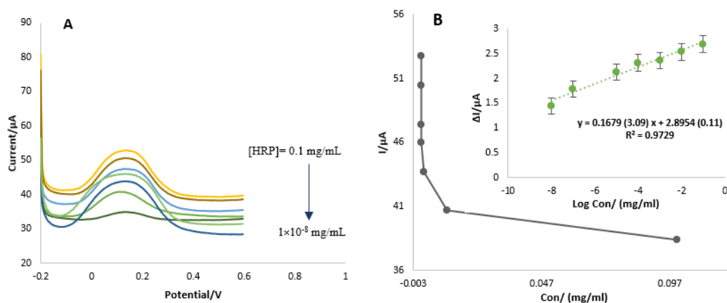
Fig. 4.20 | A) DPV of MIP/poly(Tyr)-CS/SPCE in different concentration of HRP (0.1, 10^{-2} , 10^{-3} , 10^{-4} , 10^{-5} , 10^{-7} , and 10^{-8} mg/mL in 0.01M \text{Fe}(\text{CN})_6^{3-}/\text{Fe}(\text{CN})_6^{4-} + 0.1M KCl. B) Calibration curve of the corresponding peak currents of MIP/poly(Tyr)-CS/SPCE versus concentrations of HRP ( n = 3 , SD = 2.03 ).
