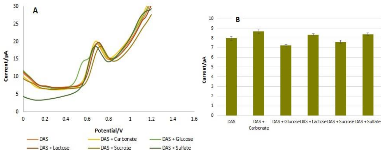
Fig. 4.7 | (A) Interference effect of lactose, sucrose, glucose, \text{SO}_4^{2-} , and \text{CO}_3^{2-} on determination of DAS by SWV method on SWCNT-COOH-SPCEs in supporting electrolyte Britton-Robinson buffer pH 5.0. (B) Histogram of interference effect.
