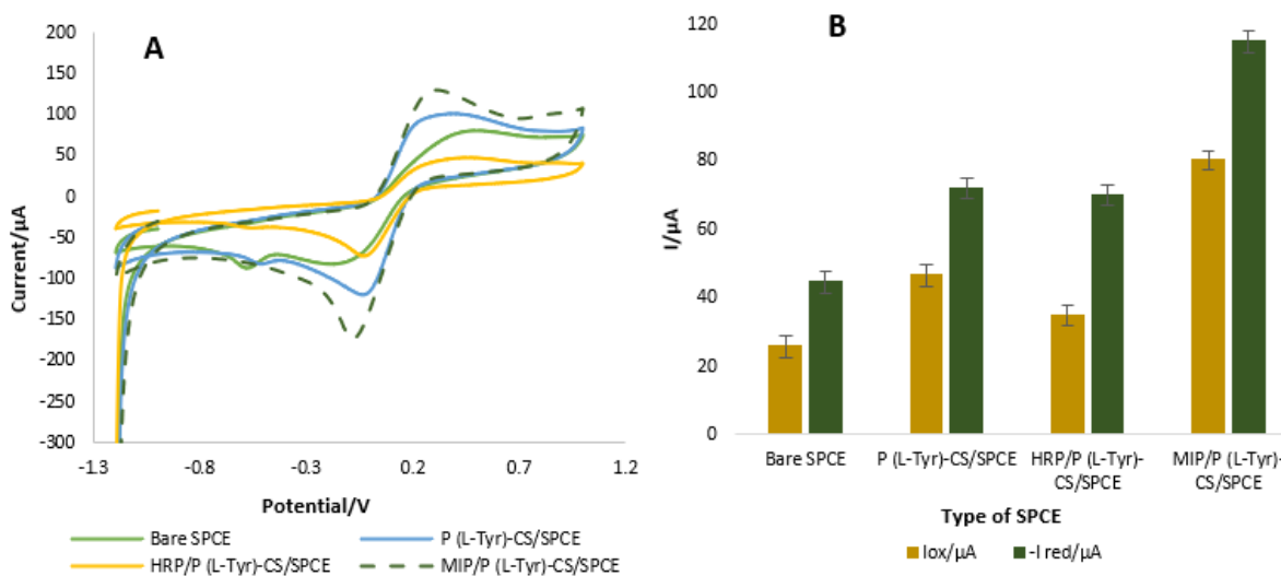
Fig. 4.18 | A) CVs of preparation steps of imprinted polymer in 0.01 M \text{Fe}(\text{CN})_6^{4-}/\text{Fe}(\text{CN})_6^{3-} +0.1 M KCl at a sweep rate of 30 mV/s. B) peak currents variation versus type of modified electrodes (n = 3, SD = 3.01).
