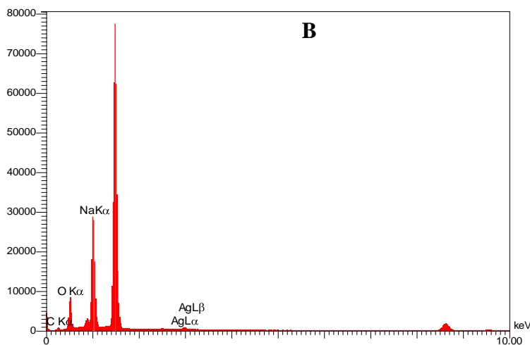
Fig. 4.8 | (A). FE-SEM images of Cit/AgNPs in various magnification. (B). EDS spectra of Cit/AgNPs.
