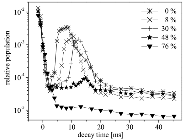
Fig. 2. Profiles of populations at N_2^+ ( B \ ^2\Sigma_u^+, v = 0 ) level during the post-discharge for selected argon concentrations in the gas mixture at a wall temperature of 300 K.
