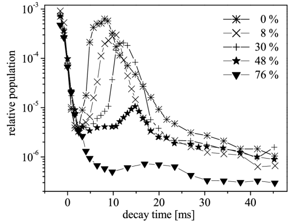
Fig. 4. Profiles of populations at levels v = 2 (a-top), v = 11 (b-middle), and v = 17 (c-bottom) of N_2 ( B \ ^3\Pi_g ) state during the post-discharge for selected argon concentrations in the gas mixture at a wall temperature of 300 K.
