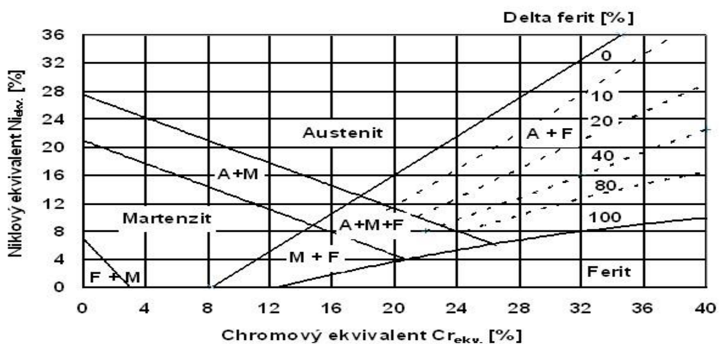
Obr. 1 Schaefflerov diagram [3].
