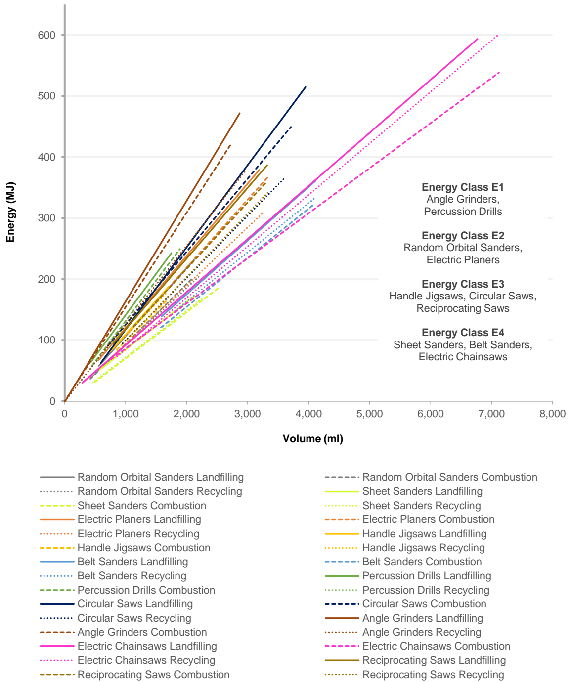
Fig. 6-8 Energy simulation of power tools category (Landfilling, Combustion & Recycling 90%).
