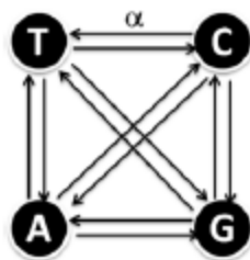
Obr. 15: Jukes-Cantor [30]
