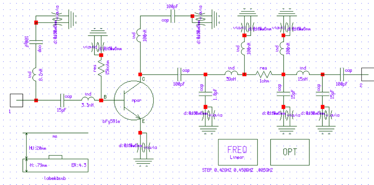
Obr. 14 Model PA
