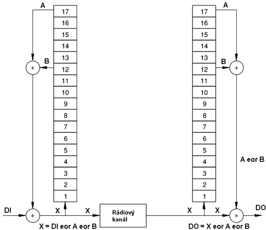
Obr. 1 Schéma scrambleru
