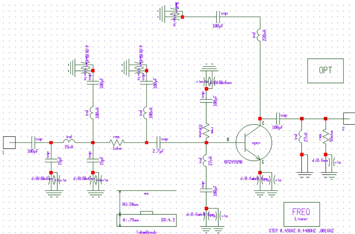
Obr. 17 Model LNA
