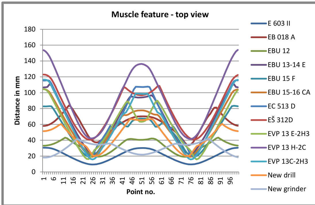
Fig. 8.39 Graph of muscle curves, top view
