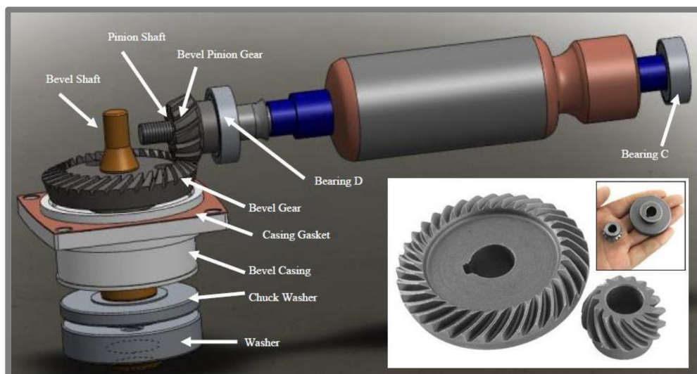
Fig. 5.9 Mechanism of an angle grinder [38]
