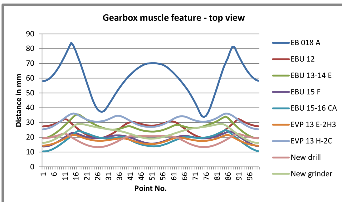
Fig. 8.40 Graph of gearbox muscle shapes, top view
