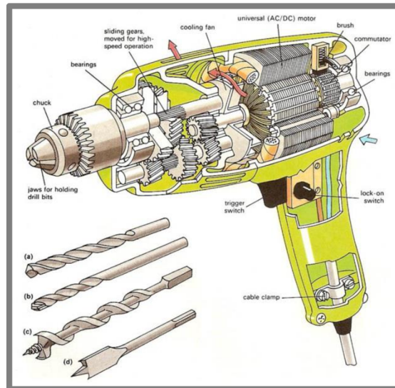
Fig. 5.5 Section through corded drill [37]
