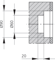
Robotic system mounting | C
