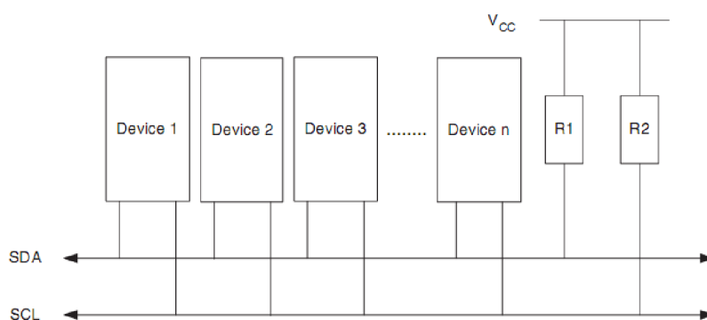
Obr. 1.1: Design I2C sběrnice [1]
