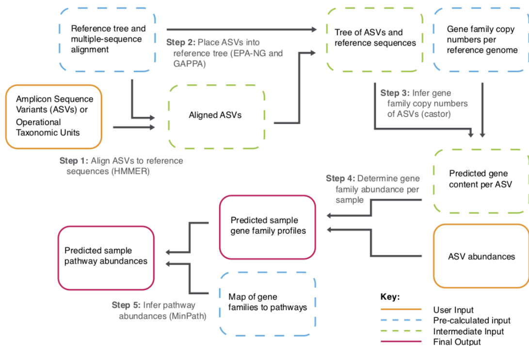
Figure 4.2: Diagram showing the workflow of Picrust2. This picture is originally from the wiki of Picrust2 [10]
