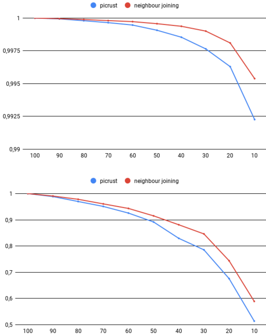
Figure 6.16: Comparison of my implementation of Picrust with my the results from my tool. The upper chart shows evaluation on all bacterial functions, the graph below on the rarest 1% of bacterial functions. The x-axis represents the ratio of known profiles in the sample, the y-axis represents the correlation between expected and computed result.
