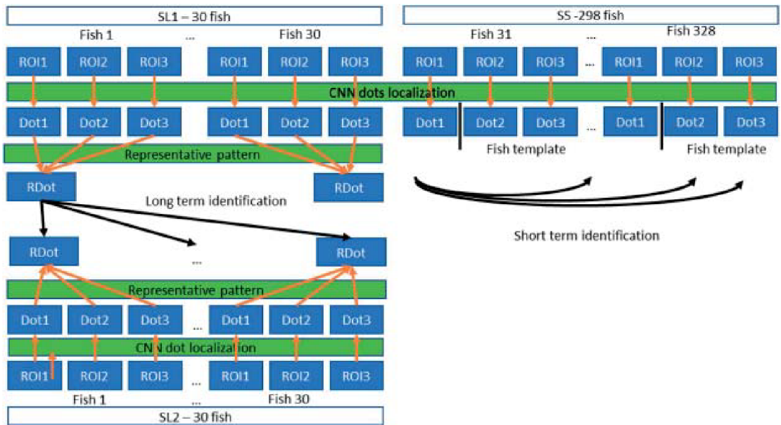
Figure 6. Scheme of dot localization-based approach to identification. The dots (Dot) for each ROI of each fish are detected using CNN. The dots are used for short-term identification, where two images are used as the pattern and one image as an unknown image. The representative dot pattern (RDot) is calculated for each fish from all fish dot patterns. The representative dot pattern is used for long-term identification for the SL1, SL2, SL3 and SL4 datasets.
