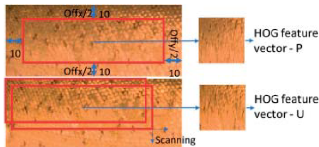
Figure 10. Similarity measure of two fish skin patterns using HOG feature descriptor. Upper row (P)—image of the identified fish. The subpart of the pattern is used for parametrization. The subpart is normalized to a 64 \times 64 pixel image, and the HOG feature vector is calculated. Bottom row (U)—images of the unknown fish. The subpart of the pattern is selected from the image repeatedly by scanning over the image. The subpart is normalized to a 64 \times 64 pixel image, and the HOG feature vector is calculated. The similarity between the P and U images is the best similarity between the P subset and one of the U subsets from the scanning.
