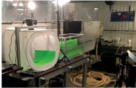
Figure 1. Experimental setup for data collection. Photo tent with camera installed on top, aquarium with the camera installed in front of it, and LED lights for scene illumination. The green background was installed in the tent and aquarium.
