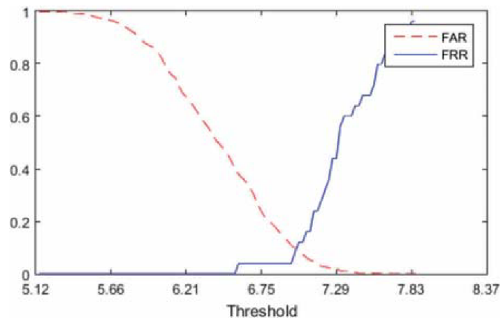
Fig. 5 FAR-FRR diagram. The change of correctly and incorrectly identified individuals
