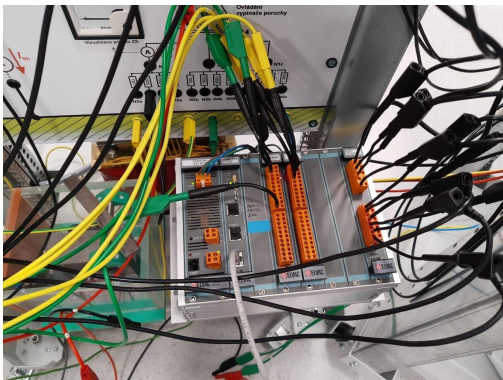
RTU7M-8, Elvac
