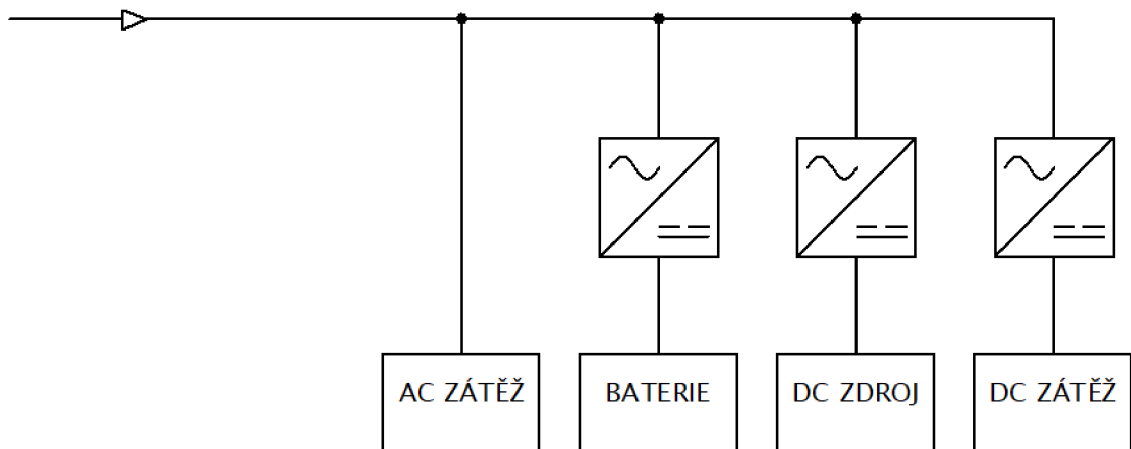
Obr. 2-11 AC coupling [6]
