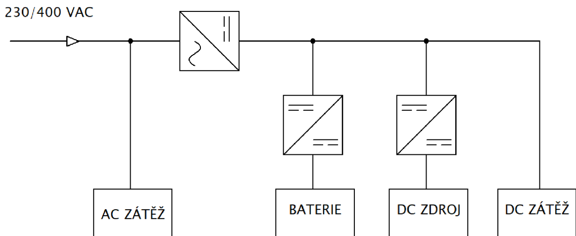
Obr. 2-10 DC coupling [6]
