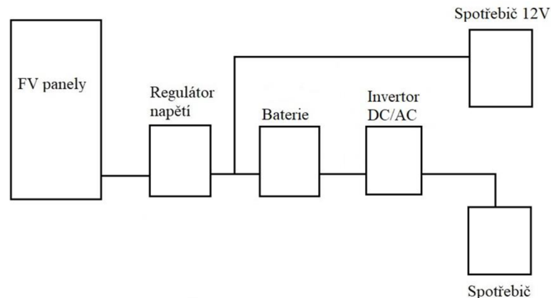
Obr. 2-5 Off-grid systémy
