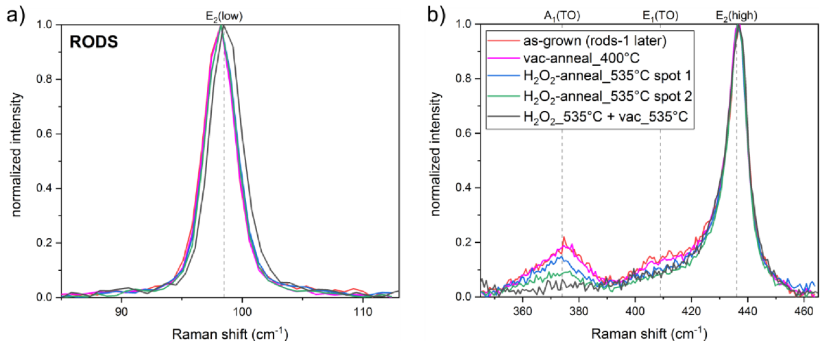
Fig. 32: Combined effect of annealing temperature and environment. Normalized Raman spectra of a) ZnO E_2(\text{low}) peak and b) ZnO E_2(\text{high}) peak for samples annealed in vacuum (400 °C, 535 °C), \text{H}_2\text{O}_2 atmosphere (535 °C) and as-grown.
