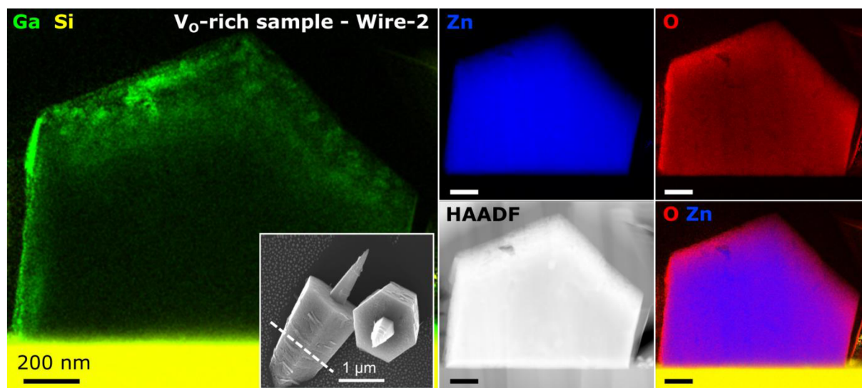
Fig. 52: STEM EDS maps of Wire-2 lamella from the V_0 -rich sample. The location of the lamella (cut perpendicularly to the growth substrate) is shown in the inset (SEM top view, white dashed line) and also in Fig. 50a. Results for Ga, Si, Zn and O elements are presented, together with HAADF image and combined O+Zn map. Imaging: K. Bukvišová. Data analysis: author of the thesis.
