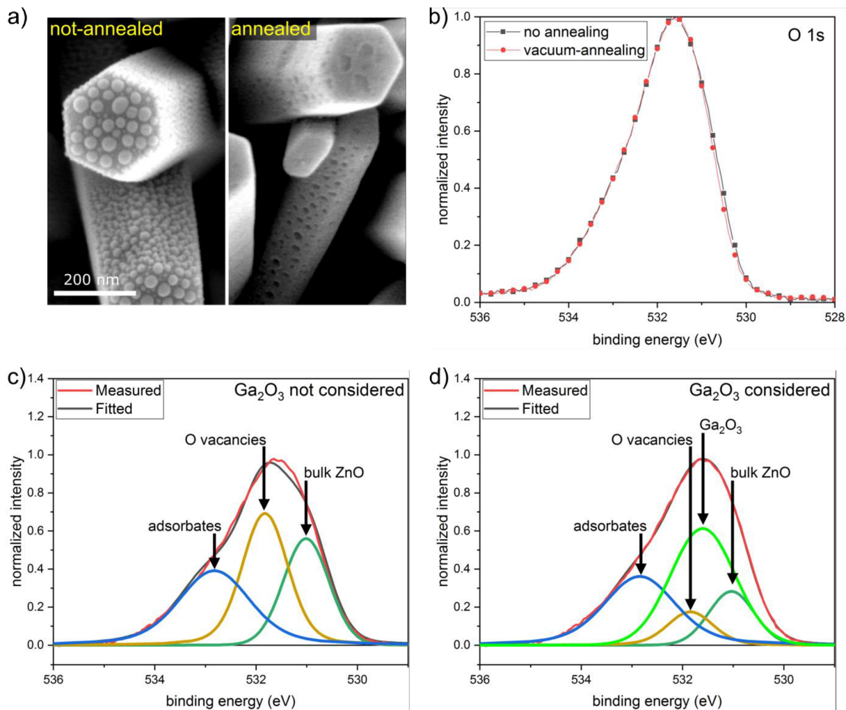
Fig. 44: a) SEM micrographs of ZnO nanowires over-deposited with Ga (at room temperature) and either taken out of the vacuum chamber directly (left, no annealing step) or annealed in vacuum at 535 °C upon Ga deposition and only then taken out (right). b) Detailed XPS spectra of O 1s peak of these samples. Interestingly, no difference is observed. c) Deconvolution of the O 1s peak based on the same fit-parameters as in section 3.3. The Ga 2 O 3 -component is not considered here, i.e. only the components assigned to surface adsorbates on ZnO (blue), oxygen vacancies (gold) and standard ZnO lattice (dark green) are considered. Note that the cumulative fit deviates from the measured curve, indicating the presence of another component. d) Deconvolution of the O 1s peak, taking into account also the Ga 2 O 3 -component (light green) of O 1s peak.
