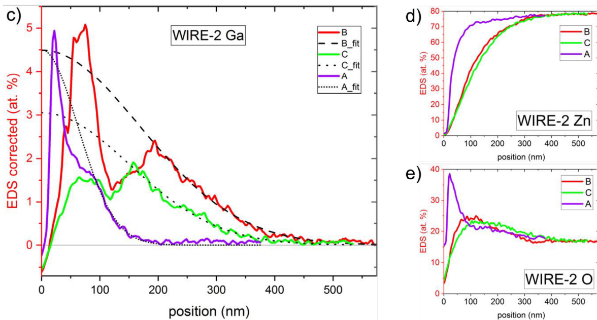
Fig. 53: ZnO Wire-2 (V 0 -rich sample) EDS profiles. a) EDS map of Ga (green) acquired from the inclined cross-sectional TEM lamella. The location of the lamella within the wire is shown in the inset (take notice of the wire facets). The position of the elemental line profiles (perpendicular to lamella's edges) is indicated by coloured dashed lines (purple, red and green for the A, B and C edge, respectively). The line spectra are integrated over a 100px-wide area, indicated by the dotted lines of the same colour. b) To illustrate the data handling, the as-measured line spectra of the B profile are shown for Ga, Zn, O and HAADF signal. No correction is applied yet (see explanation in the text). The lower graph in b) shows a zoomed-in Ga spectrum from the upper graph. c,d,e) Corrected EDS depth-profiles of gallium, zinc and oxygen, respectively. After necessary corrections described in the text, the spectra represent real depth-profiles, perpendicular to nanowire sidewall facets A, B and C. The black dashed/dotted lines in c) show the Ga concentration profiles extracted from the diffusion model for A, B and C facets. (Note a good fit for the inner part of the profiles.) Also, pay attention to different colour-coding of the b) figure, which corresponds to the EDS maps shown in Fig. 52. In contrast, the colour-coding of c-e) reflects the schematics in figure a).
