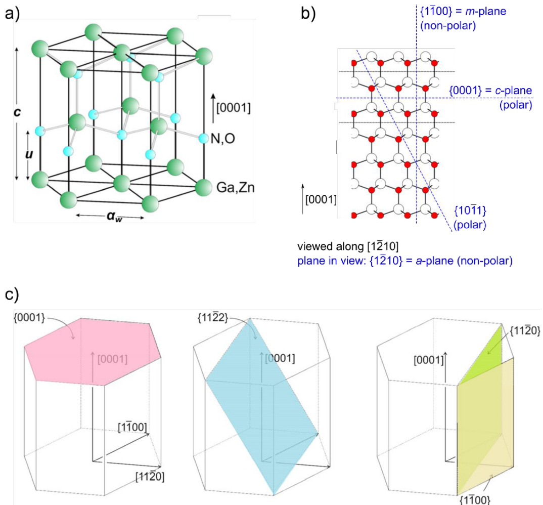
Fig. 21: ZnO crystallography. Adapted from [101]. a) Ball and stick model of the wurtzite ZnO (or GaN) structure. The a_w and c are the lattice constants; u is the displacement of the O- and Zn-sublattice along the [0001] -axis. b) Ball and stick model of wurtzite crystallographic planes. Open (filled) circles correspond to cations (anions), respectively. c) Schematic representation of selected low-index planes in the WZ crystal.
