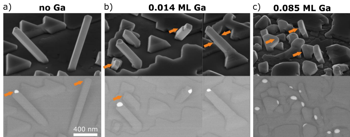
Fig. 13: Growth of Ge nanowires from Au–Ga catalyst formed during the growth. SEM images with SE contrast (top row) and BSE contrast (bottom row). The alloyed catalyst was formed by depositing gallium onto the sample with pure Au catalysts on top of previously grown Ge nanowires. The series shows the effect of deposition of different amount of gallium. The areas of interest are highlighted by orange arrows.
