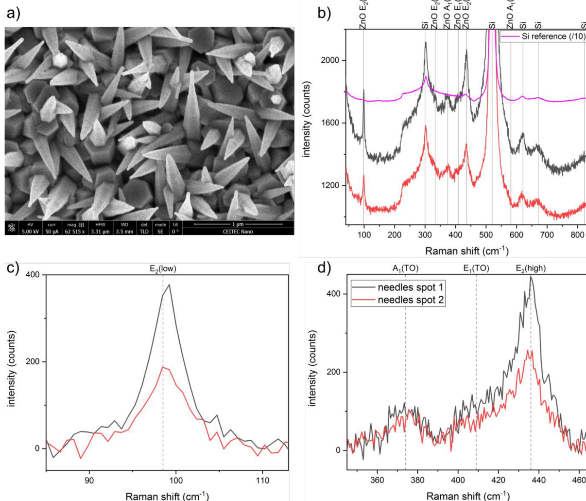
Fig. 29: ZnO needle-like nanowires. a) SEM top-view image. b) As-measured Raman survey spectra taken at different positions. Si growth substrate measurement included (purple; signal intensity divided by a factor of 10). c,d) Detailed Raman spectra of ZnO E_2(\text{low}) and E_2(\text{high}) peaks, respectively. The legend is common for all graphs.
