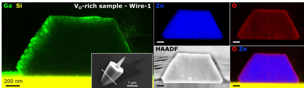
Fig. 54: STEM EDS maps of Wire-1 lamella (taken from the V_O -rich sample). The location of the lamella (cut perpendicularly to the growth substrate) is shown in the inset (SEM top view, white dashed line) and also in Fig. 50b. Results for Ga, Si, Zn and O elements are presented, together with the HAADF image and combined O+Zn map. Imaging: K. Bukvišová. Data analysis: author of the thesis.
