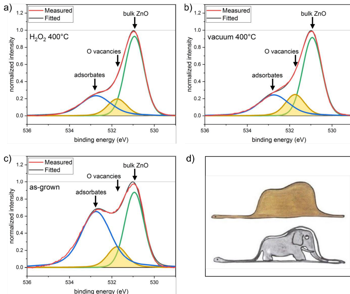
Fig. 39: Normalized XPS O 1s peak spectra of selected samples – deconvolution into individual components: bulk ZnO (green), O vacancies (gold) and surface adsorbates (blue). a) \text{H}_2\text{O}_2 -annealed sample (400 °C). b) Vacuum-annealed sample (400 °C). c) As-grown sample. d) A boa constrictor digesting an elephant. Adopted from [146].
