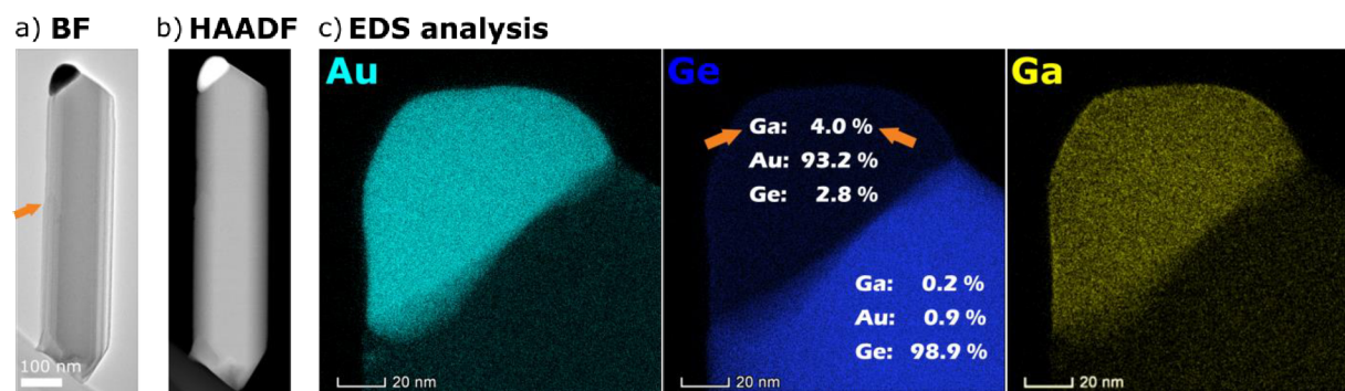
Fig. 14: a,b) TEM images (BF and HAADF contrast, respectively) of a Ge nanowire, for which an alloyed Au–Ga catalyst was formed in the middle of the growth (note the corresponding slight change in diameter, indicated by the orange arrow). A wire from the sample shown in Fig. 13b was used. c) STEM EDS analysis of this wire. The measured composition of catalyst droplet and nanowire body is inscribed. TEM imaging and EDS analysis: K. Bukvišová.
