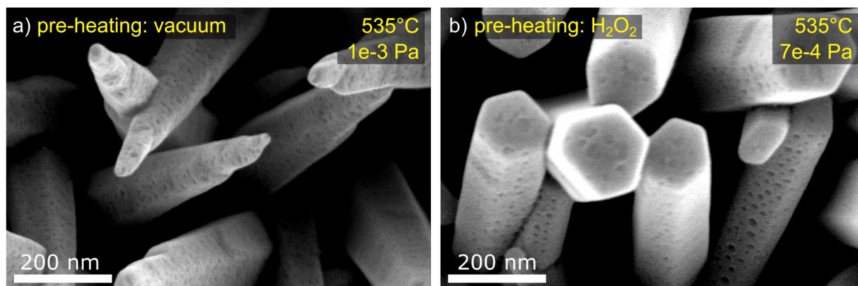
Fig. 43: Samples pre-annealed at high vacuum (a) and H 2 O 2 atmosphere (b). No morphology difference is observed wrt. nanowire damage or Ga remnants.
