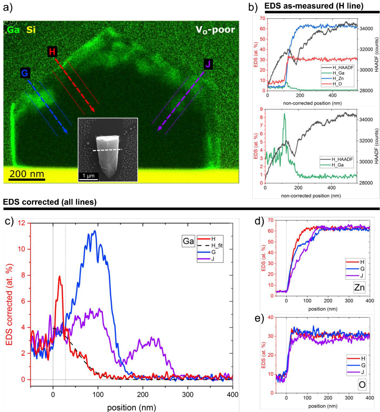
Fig. 58: EDS profiles of the V_{O} -poor nanowire. a) EDS map of Ga (green) acquired from the inclined cross-sectional TEM lamella (see its location in the SEM top-view inset). The position of the elemental line profiles (perpendicular to lamella's edges) is indicated by the coloured dashed lines. The line spectra are integrated over a 60px-wide area, indicated by the dotted lines of the same colour. b) For illustration, the as-measured line spectra of the H profile are shown for Ga, Zn, O and HAADF signal. No correction is applied yet. The lower graph in b) shows a zoomed-in Ga spectrum from the upper graph. c,d,e) Corrected EDS depth-profiles of gallium, zinc and oxygen, respectively. After the corrections described in the text, the spectra represent real depth-profiles, perpendicular to nanowire sidewall facets. In fig. c), the grey dotted vertical line (serving as a guide to the eye) separates the surface-influenced region of the H profile, which is not considered in the diffusion model. The black dashed line in c) shows the Ga concentration profile extracted from the diffusion model for H measurement. Beware of the different colour-coding of b) figure, which corresponds to the EDS maps shown in Fig. 57. In contrast, the colour-coding of c-e) reflects the schematics in fig a).
