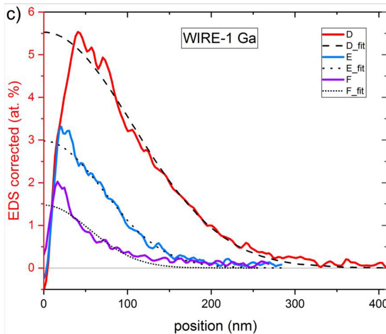
Fig. 55: ZnO Wire-1 ( V_o -rich sample) EDS profiles. (The data layout is the same as in Fig. 53 for Wire-2). a) EDS map of Ga (green) acquired from the inclined cross-sectional TEM lamella. The location of the lamella within the wire is shown in the inset (take notice of the wire facets). The position of the elemental line profiles (perpendicular to lamella's edges) is indicated by coloured dashed lines (red, blue and purple for the D, E and F edge). The line spectra are integrated over a 100px-wide area, indicated by the dotted lines of the same colour. b) To illustrate the data handling, the as-measured line spectra of the D profile are shown for Ga, Zn, O and HAADF signal. No correction is applied yet (see explanation in the text). The lower graph in b) shows a zoomed-in Ga spectrum from the upper graph. c,d,e) Corrected EDS depth-profiles of gallium, zinc and oxygen, respectively. After necessary corrections described in the text, the spectra represent real depth-profiles, perpendicular to nanowire sidewall facets D, E, F. The black dashed/dotted lines in c) show the Ga concentration profiles extracted from the diffusion model for the D, E and F facets. Pay attention to different colour-coding of b) figure, which corresponds to the EDS maps shown in Fig. 54. In contrast, the colour-coding of c-e) reflects the schematics in fig a).
