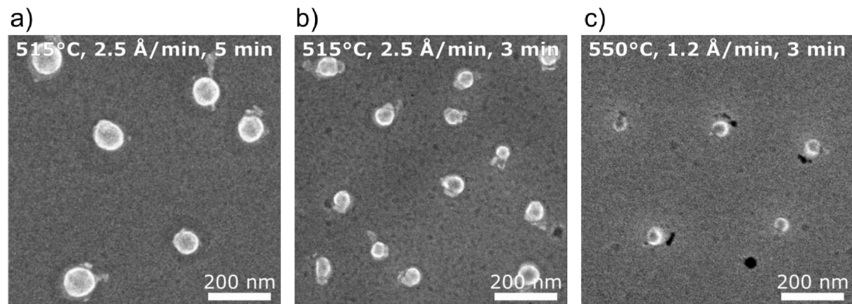
Fig. 17: SEM images of pure Al catalyst particles formed on Ge(111) wafer at various experimental conditions, controlling their size. Sample temperature during Al deposition, deposition rate and length of deposition are inscribed in each image.
