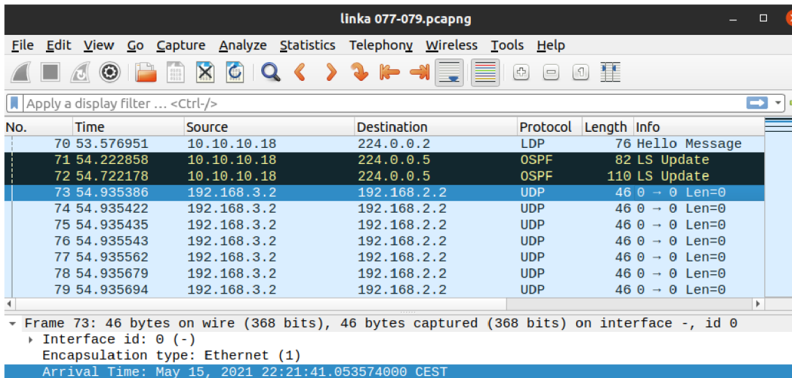
Obr. 5.6: Wireshark na linke 077-079
