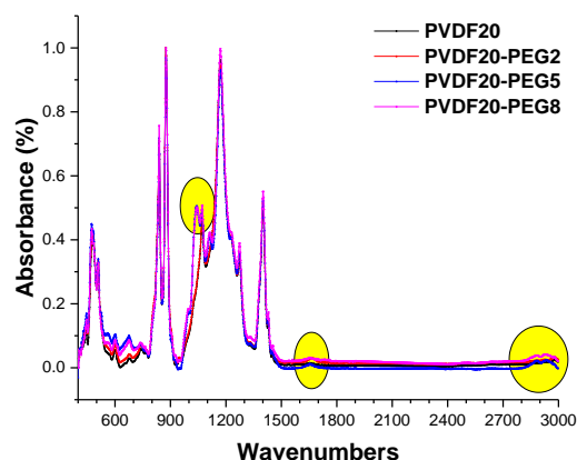
Figure 4-13 FTIR spectra of PVDF20/PEG membranes
