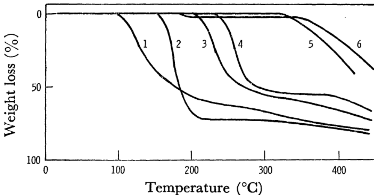
Figure 2-8 TGA thermograms of halogen-containing polymers in air [35].
