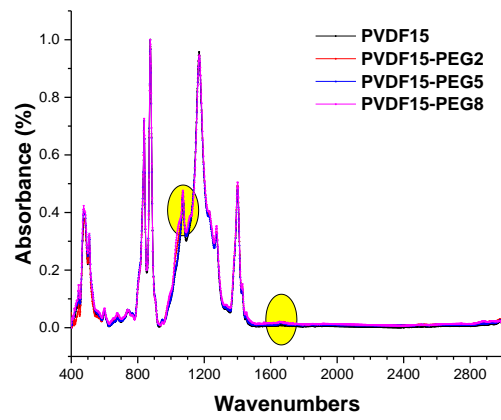
Figure 4-12 FTIR spectra of PVDF15/PEG membranes.
