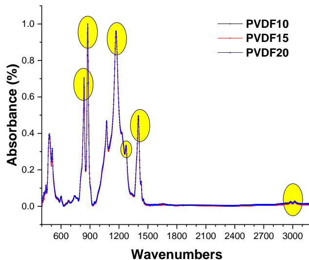
Figure 4-7 FTIR spectra of pristine PVDF membrane.
