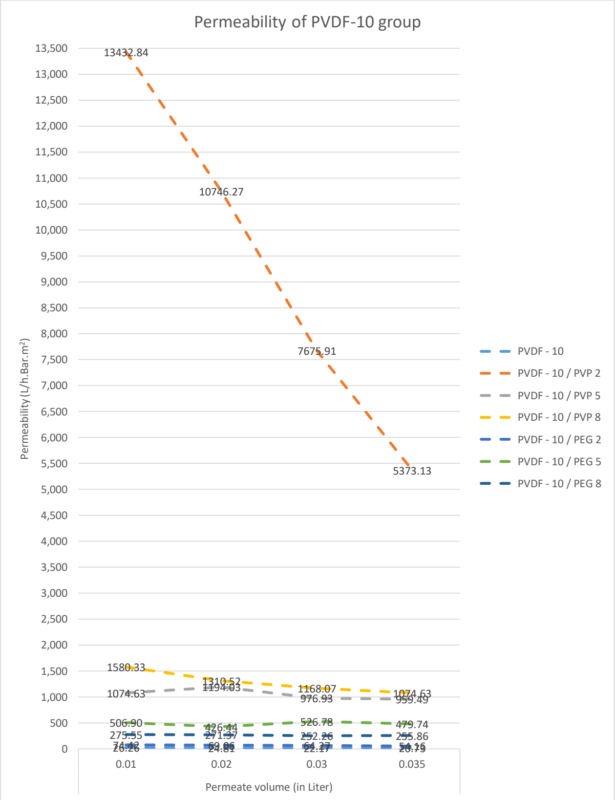
Figure 4-14 Water permeability of PVDF10 group.
