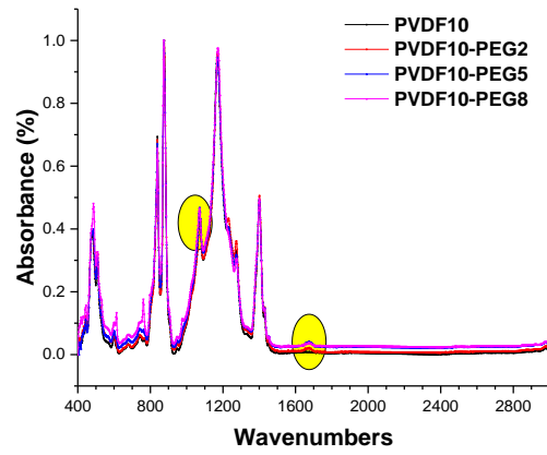
Figure 4-11 FTIR spectra of PVDF10/PEG membranes.
