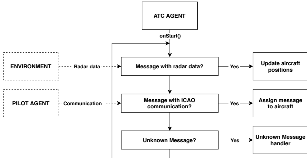
Figure 5.1: Air Traffic Control agent MessageReceiver cyclic behavior.
